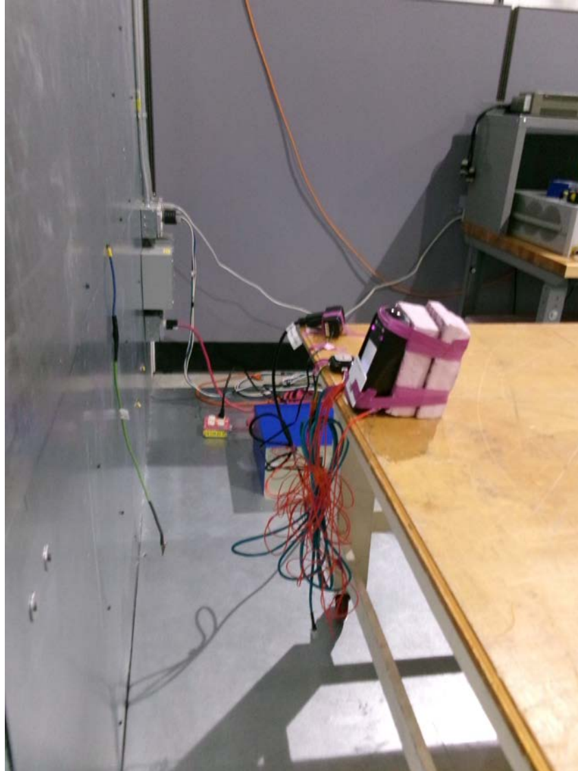
AC Line Conducted Emissions
