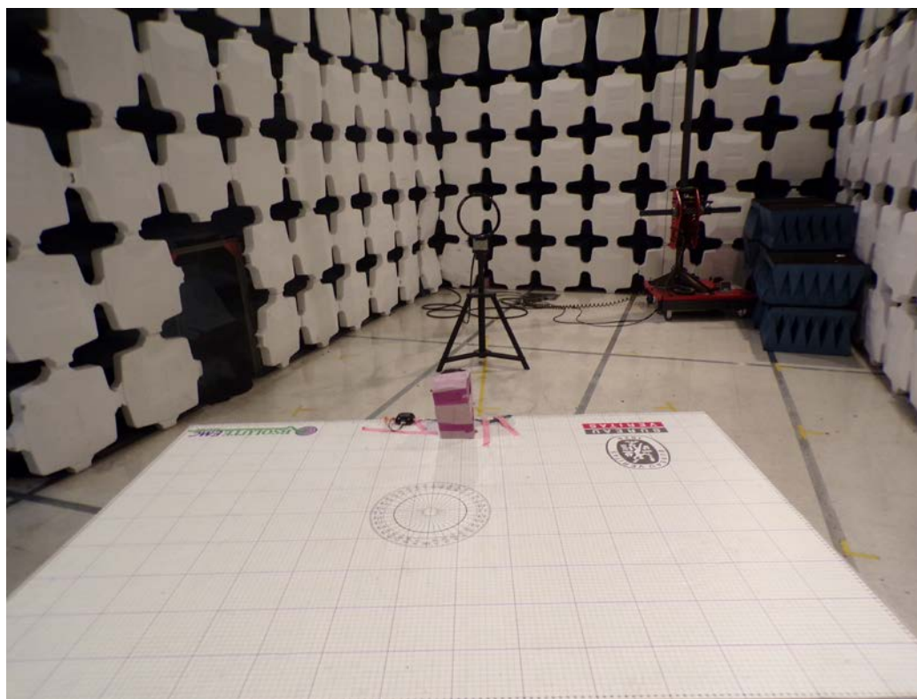
Radiated Emissions 1MHz-30MHz
