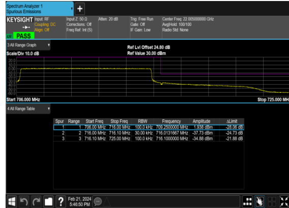
N12(10M)_DFT-s- OFDM_QPSK_Outer_Full_High_CH
