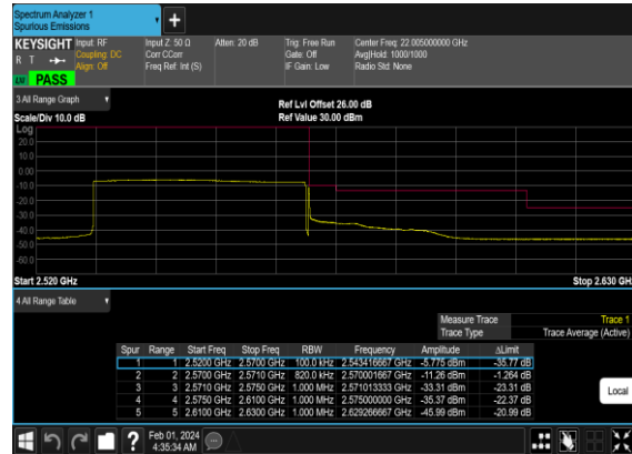
N7(40M)_DFT-s- OFDM_QPSK_Outer_Full_High_CH
