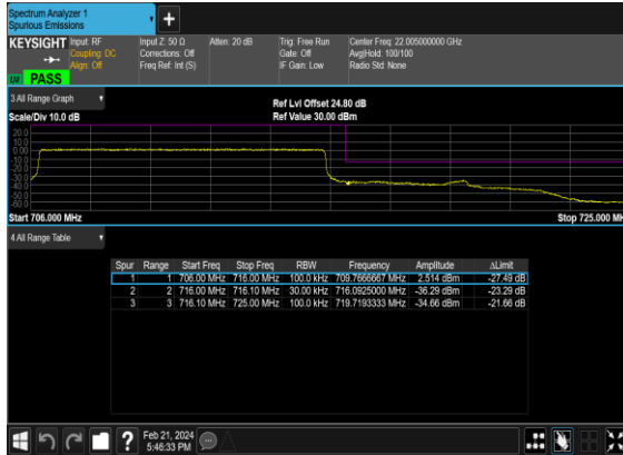
N12(10M)_DFT-s- OFDM_BPSK_Outer_Full_High_CH
