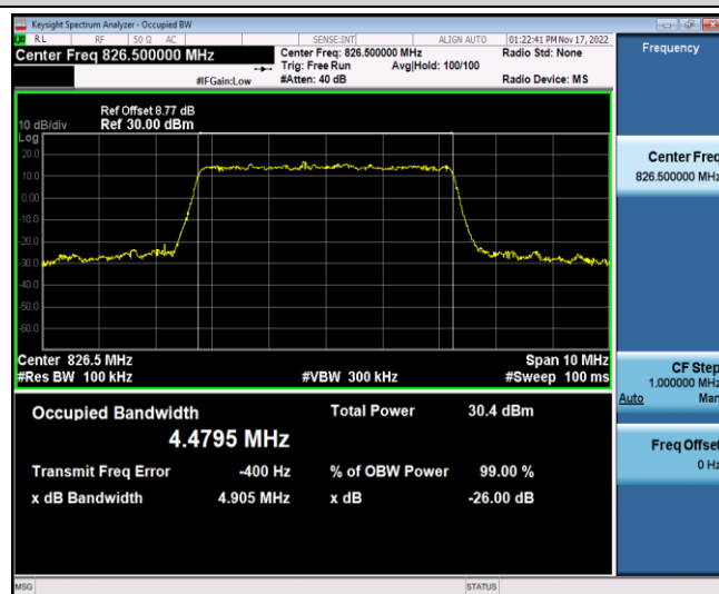
Band5-5MHz-64QAM-20625-25RB#0
