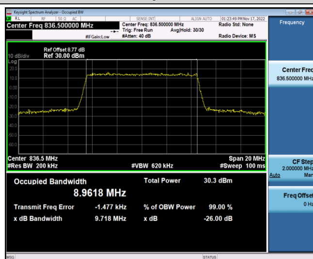
Band5-10MHz-64QAM-20525-50RB#0
