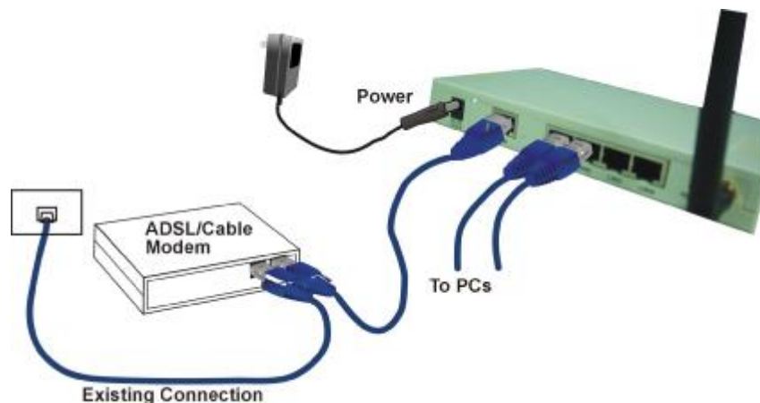
Figure 4: Installation Diagram
