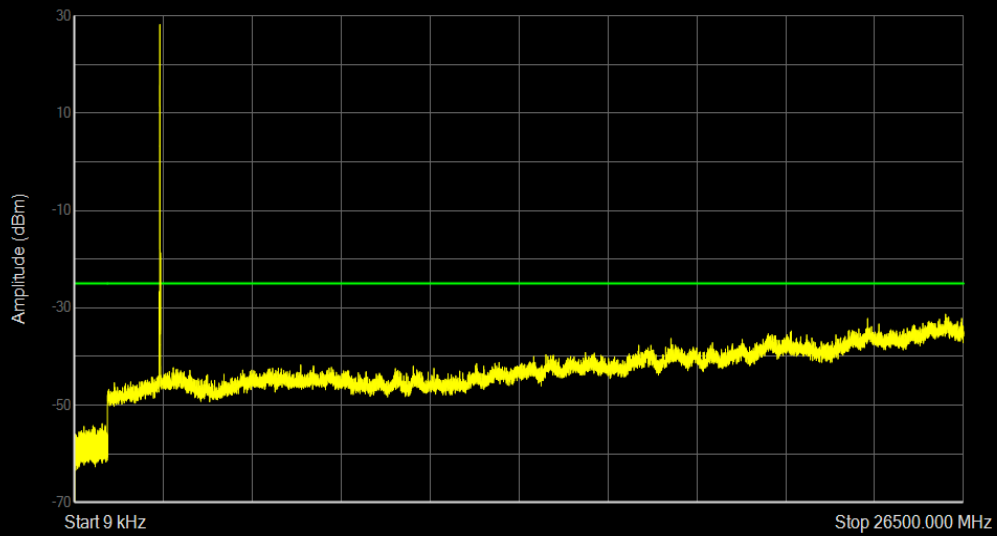
Band7 QPSK BW=10MHz Channel=21400 RB Size=1 Position=#0
