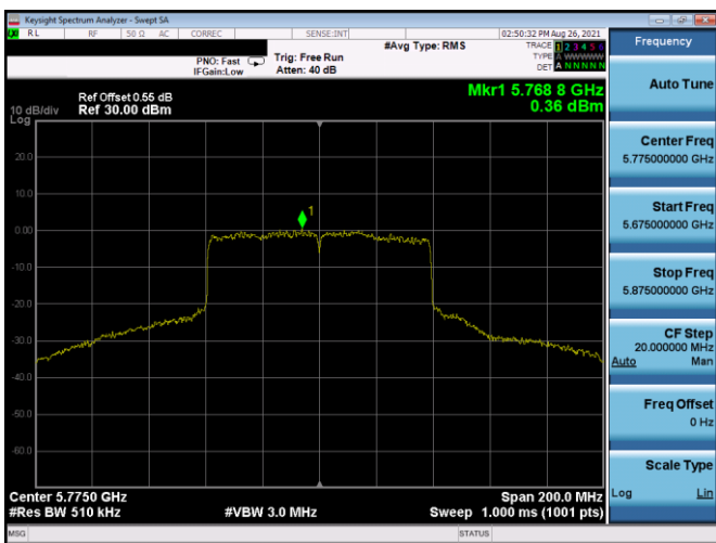
Plot 7-456. PSD Antenna 1b (80MHz BW 802.11ax(SU) – Ch. 155, MCS2)
