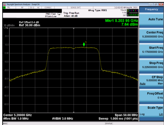
Plot 7-434. PSD Antenna 1b (20MHz BW 802.11ax(SU) – Ch. 40, MCS5)
