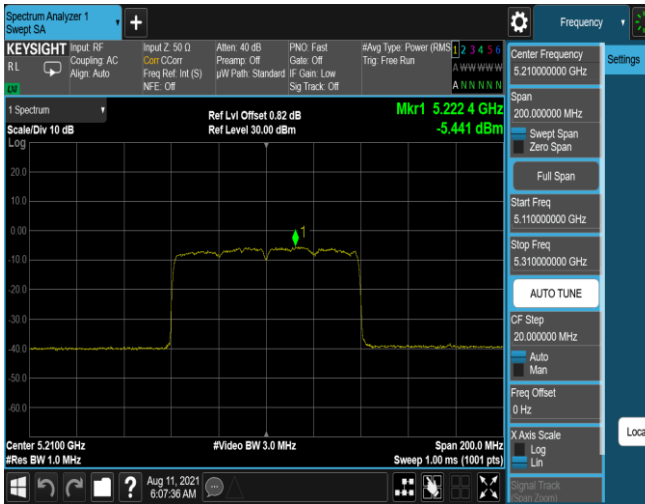
Plot 7-438. PSD Antenna 1b (80MHz BW 802.11ax(SU) – Ch. 42, MCS5)
