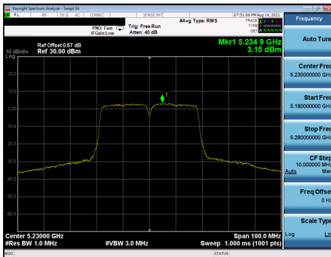
Plot 7-483. ISED PSD Antenna 1b (40MHz BW 11n - Ch.46, MCS5)
