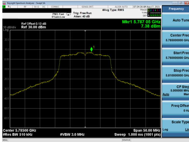
Plot 7-451. PSD Antenna 1b (20MHz BW 802.11n – Ch. 157, MCS2)
