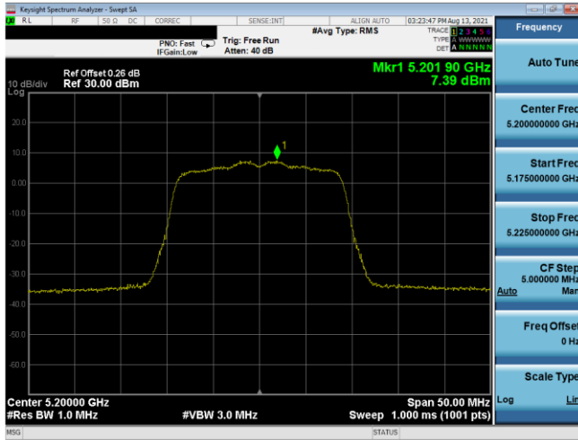
Plot 7-487. PSD SDM Antenna 5T (20MHz BW 802.11n – Ch. 40, MCS10)
