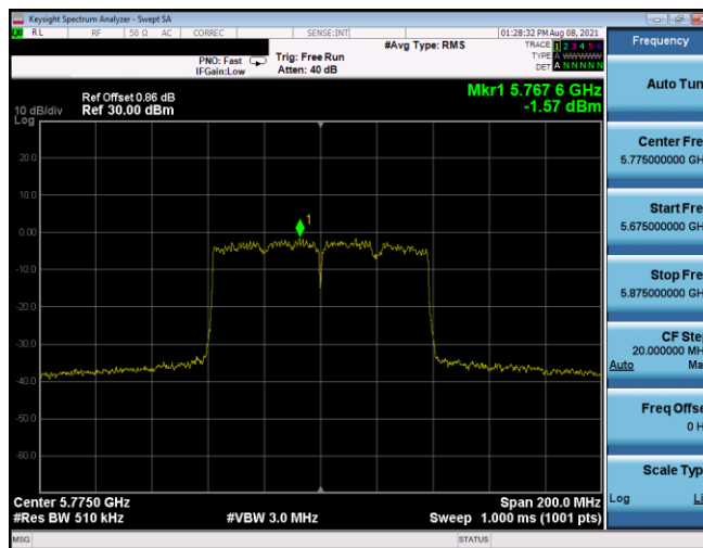
Plot 7-467. PSD Antenna 1b (80MHz BW 802.11ac – Ch. 155, MCS5)
