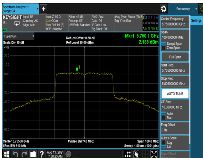
Plot 7-466. PSD Antenna 1b (40MHz BW 802.11ax(SU) – Ch. 151, MCS5)
