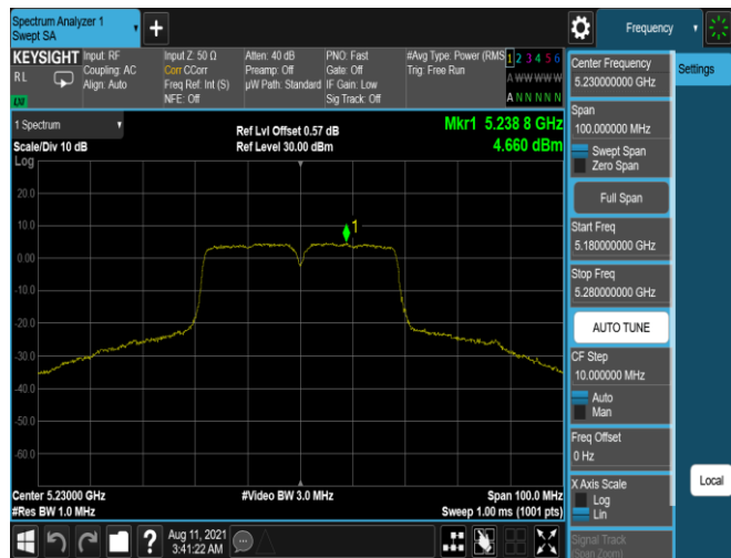
Plot 7-435. PSD Antenna 1b (40MHz BW 802.11n – Ch. 46, MCS5)
