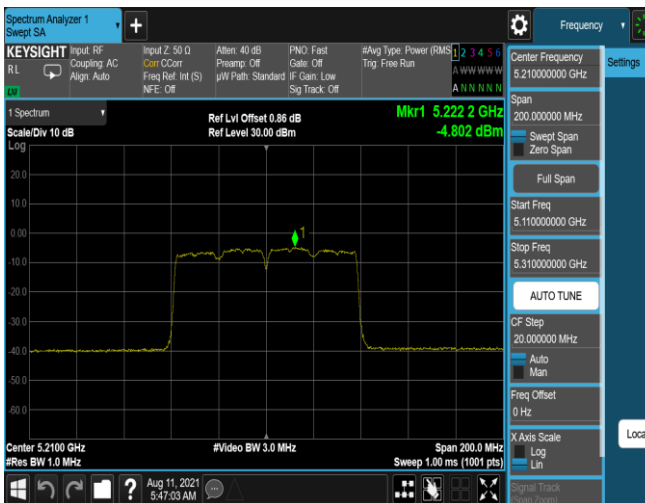
Plot 7-437. PSD Antenna 1b (80MHz BW 802.11ac – Ch. 42, MCS5)
