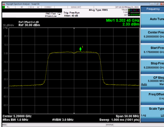
Plot 7-482. ISED PSD Antenna 1b (20MHz BW 11ax(SU) - Ch.40, MCS5)
