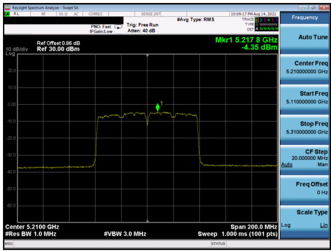
Plot 7-485. ISED PSD Antenna 1b (80MHz BW 11ac - Ch.42, MCS5)
