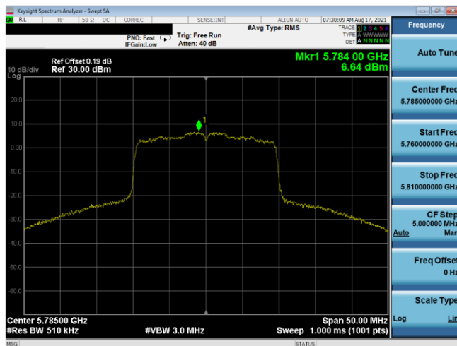
Plot 7-452. PSD Antenna 1b (20MHz BW 802.11ax(SU) – Ch. 157, MCS2)
