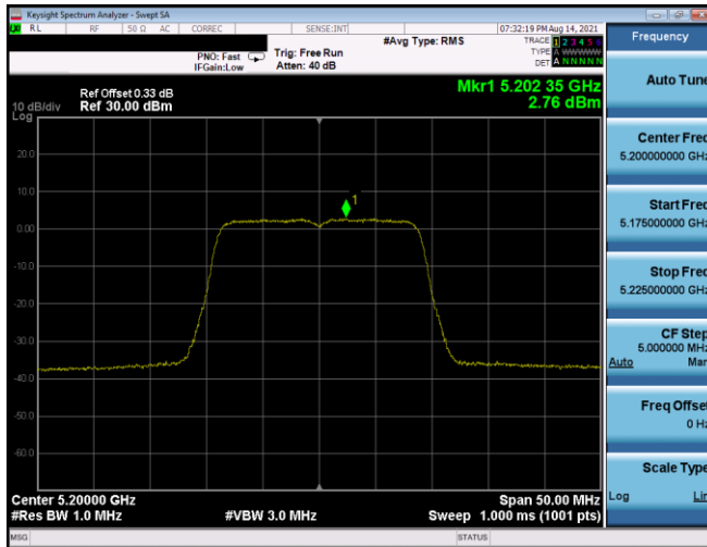
Plot 7-481. ISED PSD Antenna 1b (20MHz BW 11n - Ch.40, MCS5)
