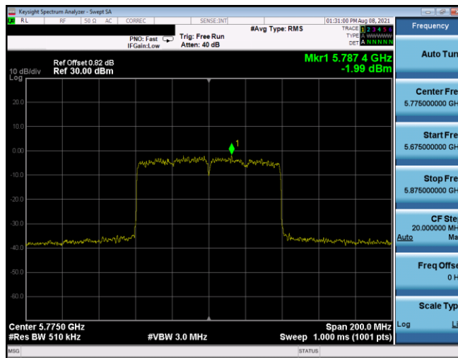
Plot 7-468. PSD Antenna 1b (80MHz BW 802.11ax(SU) – Ch. 155, MCS5)
