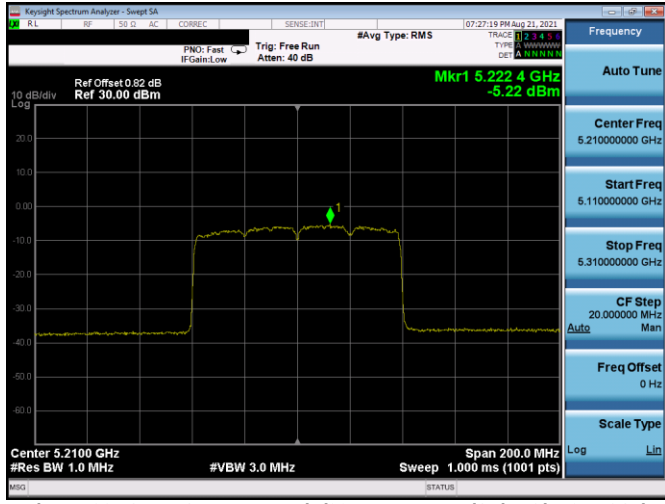
Plot 7-486. ISED PSD Antenna 1b (80MHz BW 11ax(SU) - Ch.42, MCS5)
