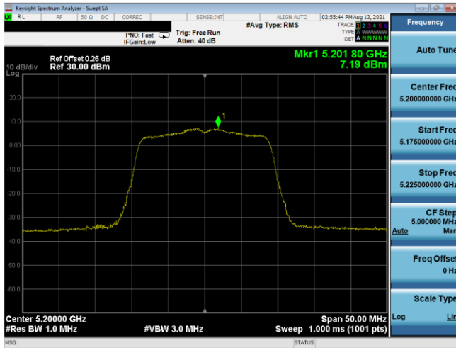
Plot 7-488. PSD SDM Antenna 3b (20MHz BW 802.11n – Ch. 40, MCS10)
