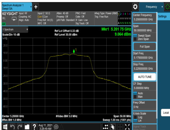
Plot 7-433. PSD Antenna 1b (20MHz BW 802.11n – Ch. 40, MCS5)
