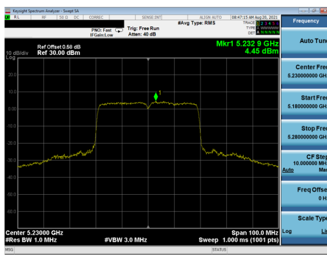
Plot 7-436. PSD Antenna 1b (40MHz BW 802.11ax(SU) – Ch. 46, MCS5)
