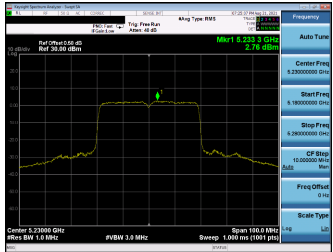
Plot 7-484. ISED PSD Antenna 1b (40MHz BW 11ax(SU) - Ch.46, MCS5)
