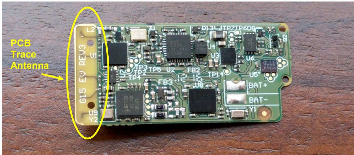
Figure 1 – EUT Internal Photo - Front
