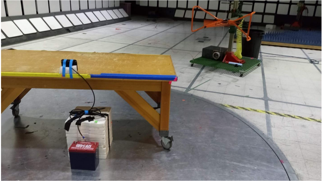
30 MHz – 1 GHz Test Setup
