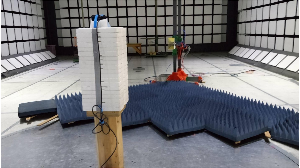
1 – 18 GHz Test Setup
