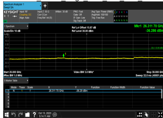
N78(60M)_DFT-s- OFDM BPSK Edge 1RB Left Low CH
