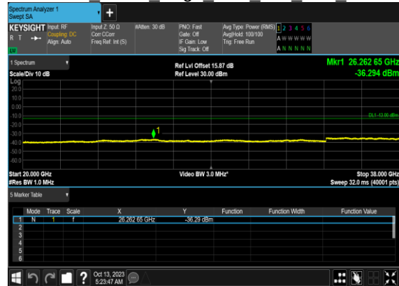
N78(80M)_DFT-s- OFDM BPSK Edge 1RB Left Low CH
