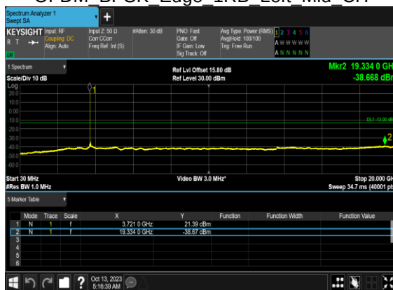
N78(60M)_DFT-s- OFDM BPSK Edge 1RB Left Mid CH
