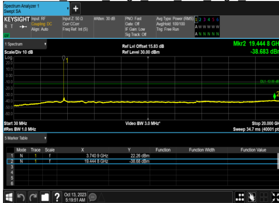
N78(60M)_DFT-s- OFDM BPSK Edge 1RB Left High CH
