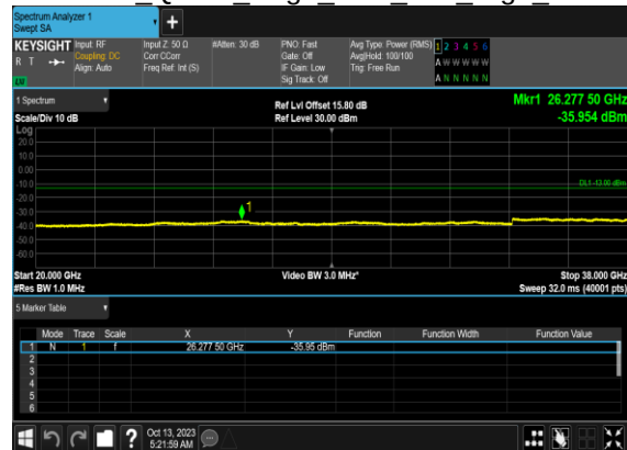
N78(60M)_DFT-s- OFDM QPSK Edge 1RB Left High CH
