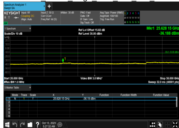
N78(80M)_DFT-s- OFDM BPSK Edge 1RB Left Mid CH
