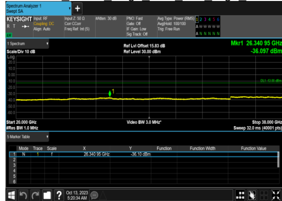
N78(60M)_DFT-s- OFDM BPSK Edge 1RB Left High CH
