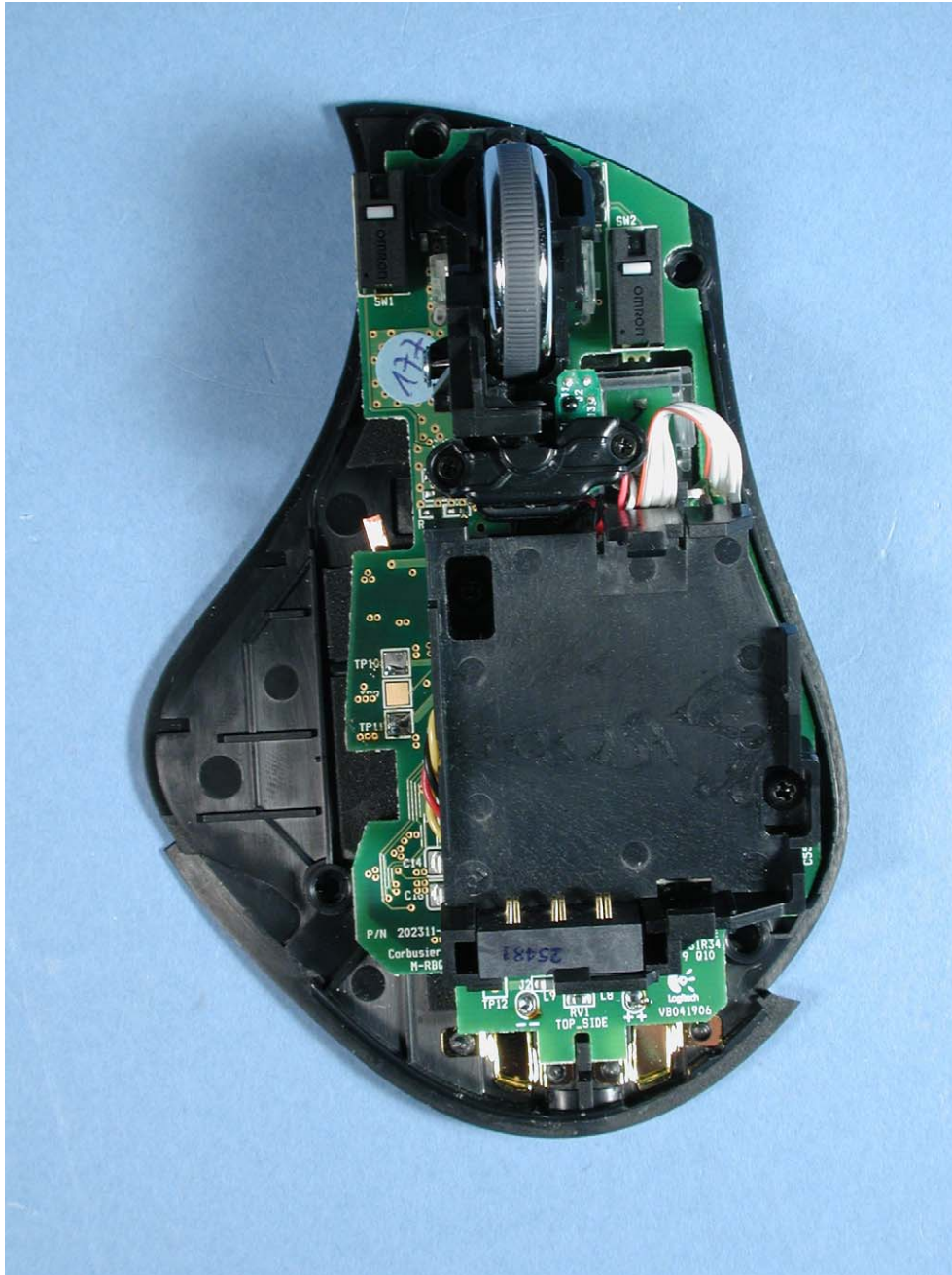
Photograph 2: M-RBQ124 internal view of bottom part
