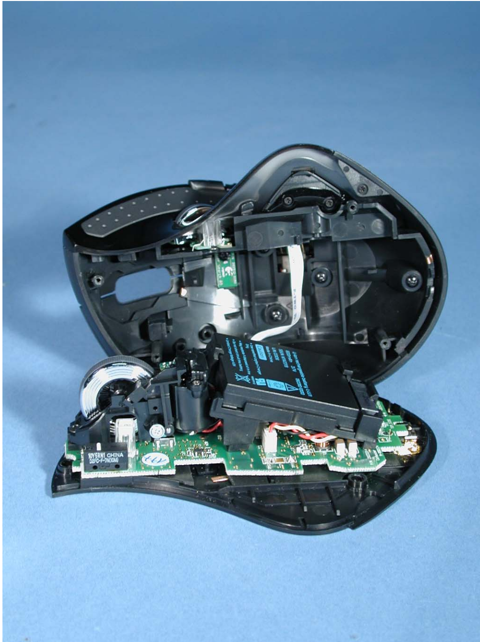
Photograph 1: M-RBQ124 exploded view
