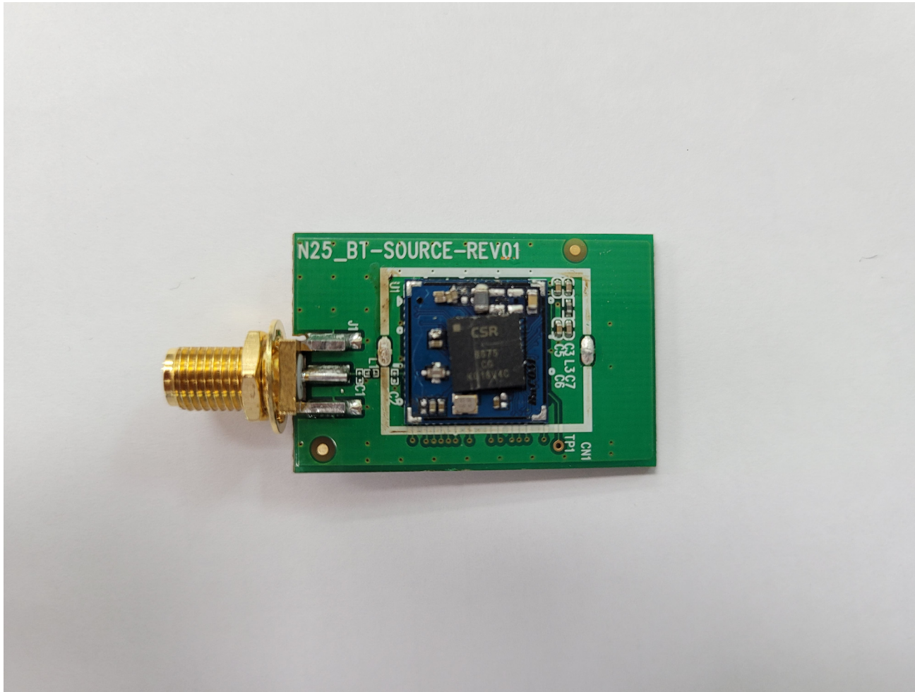
[Main board(Top)]
