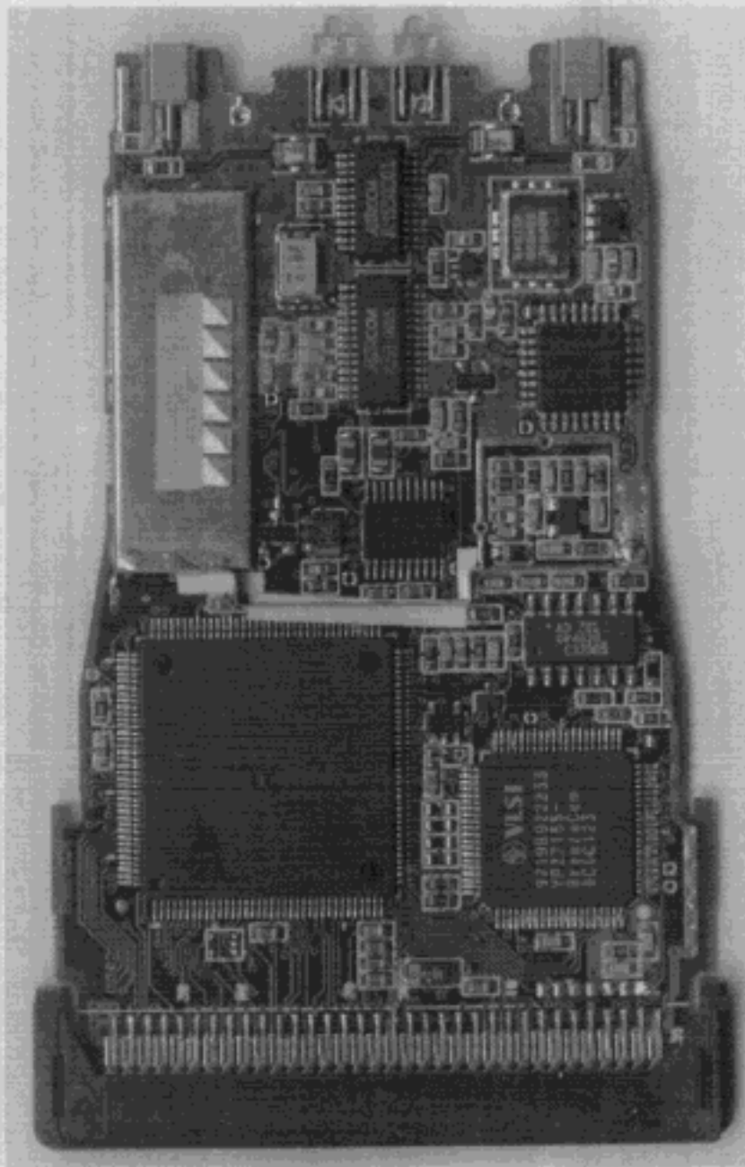
Photograph No.5 SA-PCD adapter PCB
