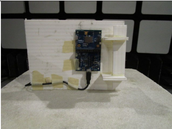
EUT Vertical – Trace Antenna
