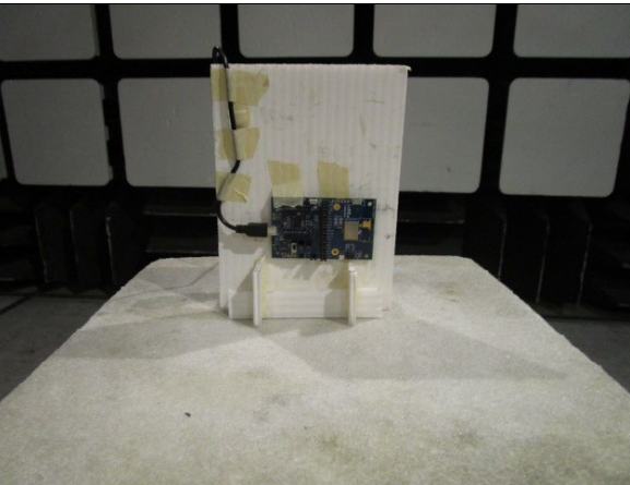
EUT Horizontal – Trace Antenna
