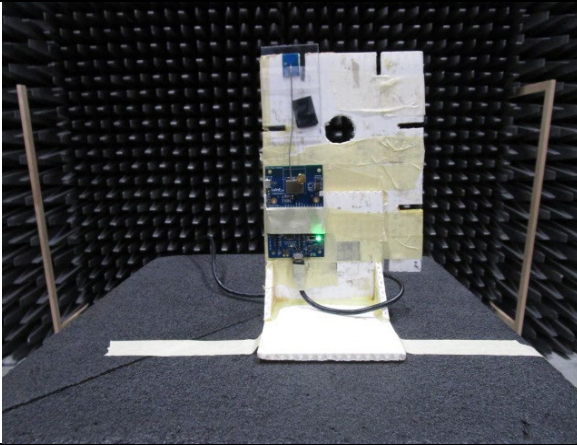
EUT Vertical – External Antenna
