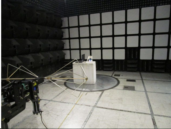
Below 1 GHz Radiated Setup
