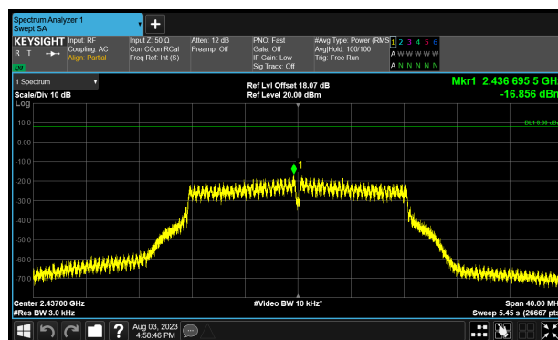
P1 2437 MHz (CH6)
