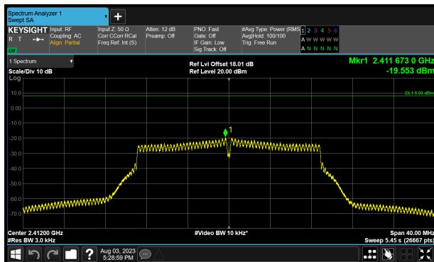
P1 2412 MHz (CH1)
