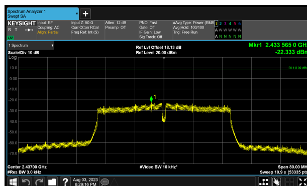
P1 2437 MHz (CH4)
