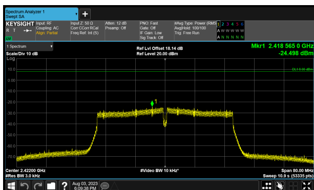
P1 2422 MHz (CH1)
