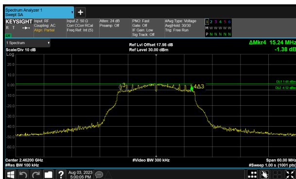
P1 (1) 2462 MHz (CH11) 6 dB Bandwidth
