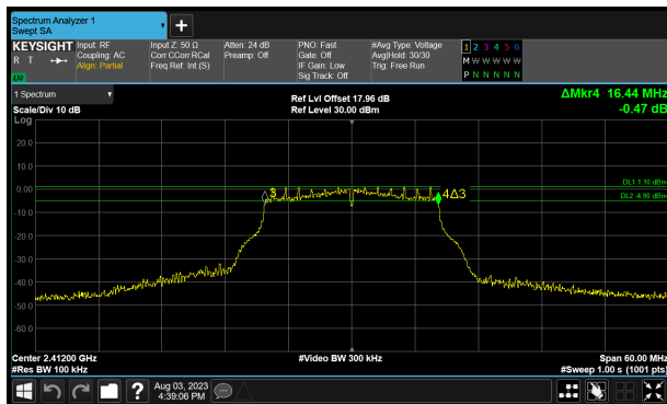
P1 (1) 2412 MHz (CH1) 6 dB Bandwidth
