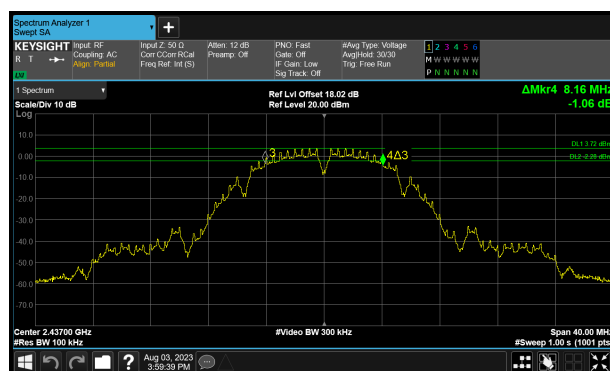
P1 (1) 2437 MHz (CH6) 6 dB Bandwidth
