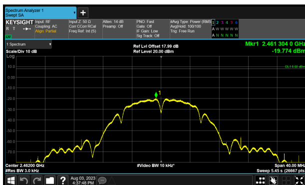
P1 2462 MHz (CH11)
