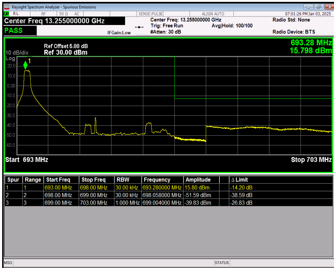
Band71 16QAM BW=5MHz Channel=133447 RB Size=1 Position=#Max
