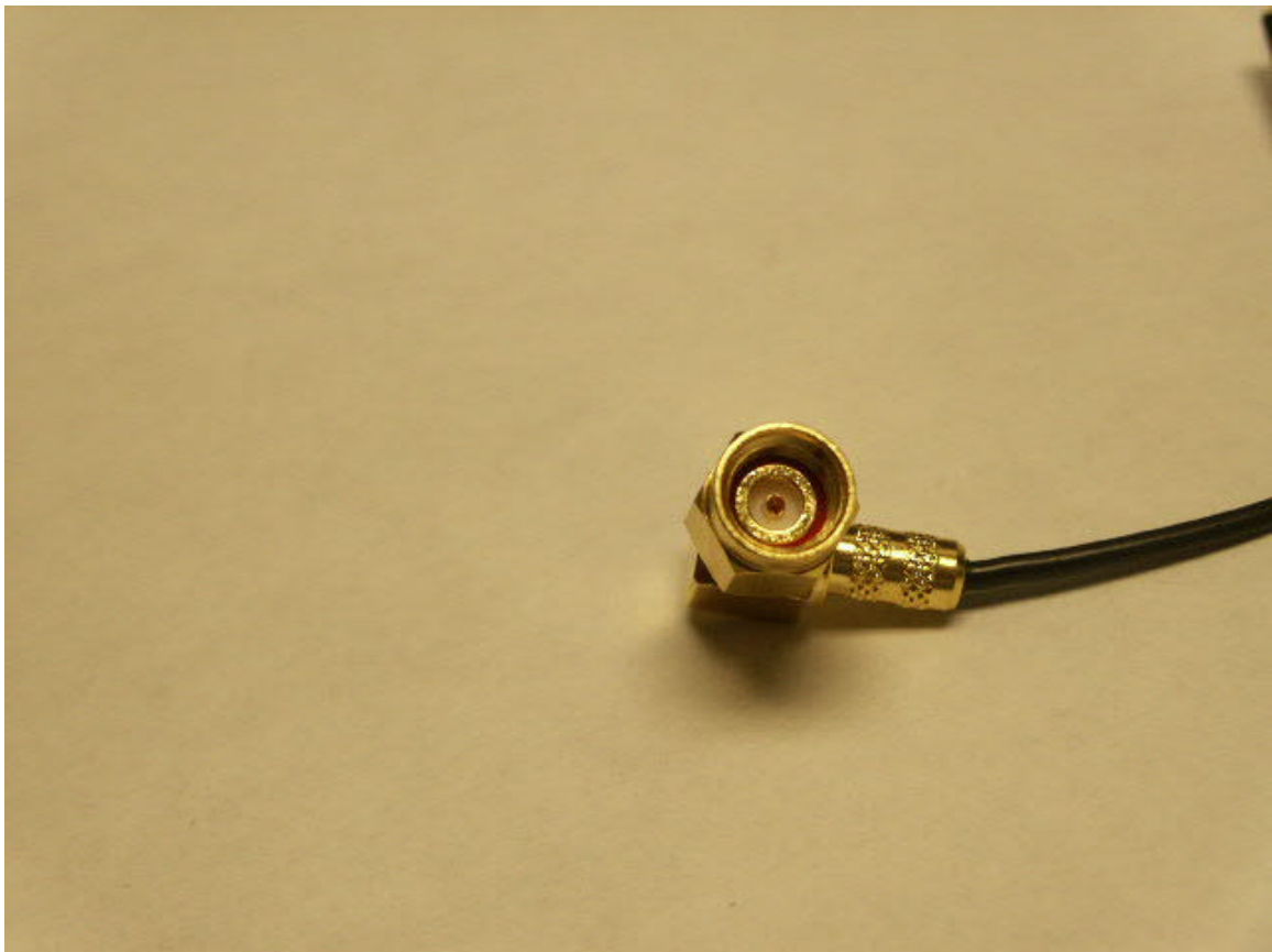
Reverse sex SMA connector
