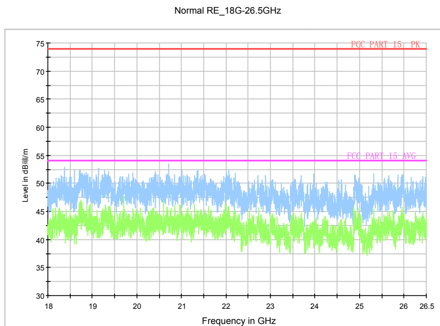
Fig.67. Radiated emission: GFSK, 18 GHz - 26 GHz
