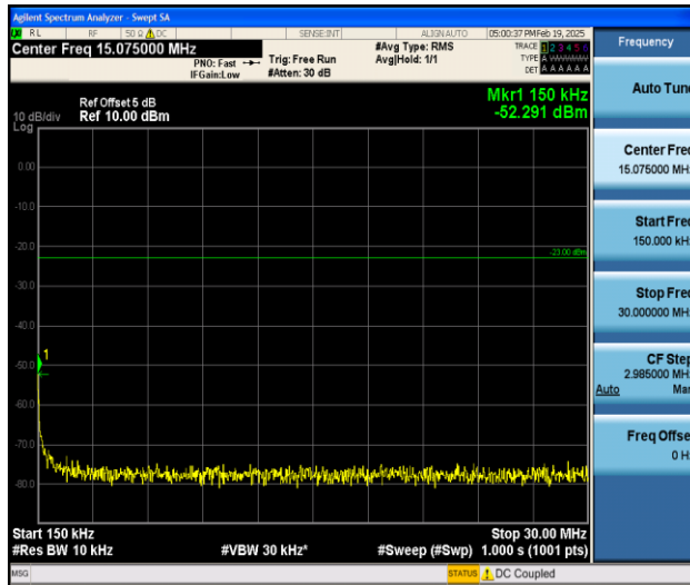
Band5_1.4MHz_QPSK_20643_1RB#0_0.15~30_0.15~30
