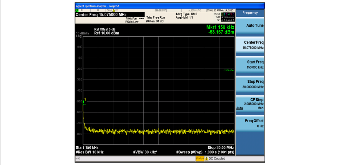
Band5_1.4MHz_16QAM_20643_1RB#0_0.15~30_0.15~30
