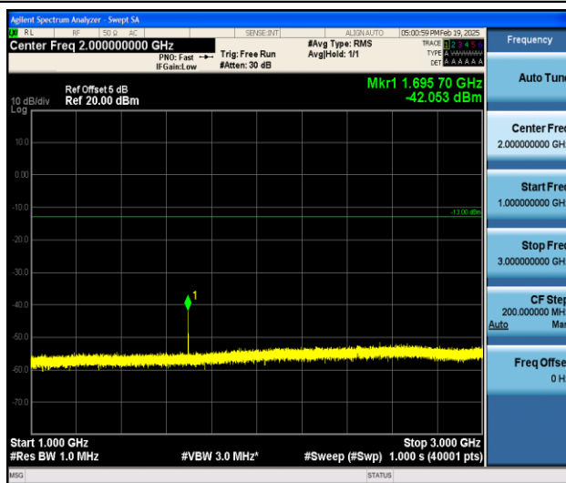
Band5_1.4MHz_QPSK_20643_1RB#0_1000~3000_1000~3000
