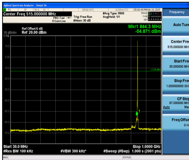
Band5_1.4MHz_QPSK_20643_1RB#0_30~1000_30~1000
