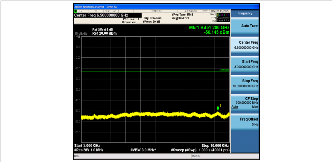
Band5_1.4MHz_QPSK_20643_1RB#0_3000~10000_3000~10000
