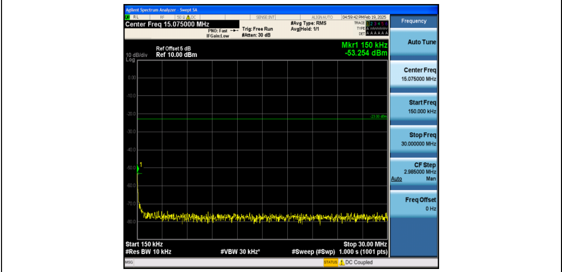
Band5_1.4MHz_16QAM_20525_1RB#0_0.15~30_0.15~30
