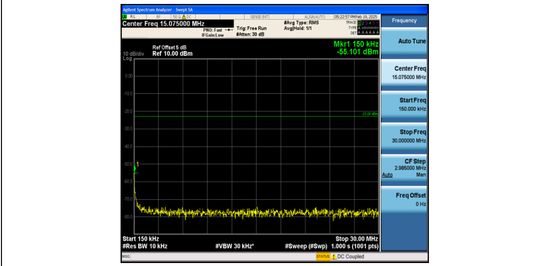
Band5_3MHz_16QAM_20525_1RB#0_0.15~30_0.15~30
