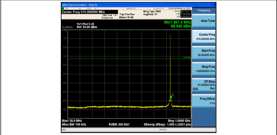
Band5_1.4MHz_16QAM_20525_1RB#0_30~1000_30~1000
