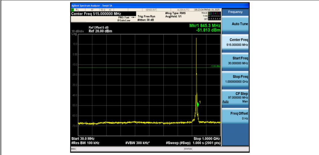
Band5_3MHz_16QAM_20525_1RB#0_30~1000_30~1000
