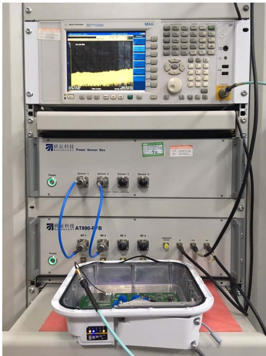
Photograph - Conducted Test Setup
