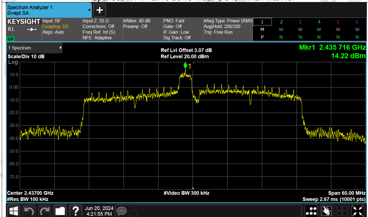
Tx. Spurious NVNT ax40 26RU Index 8 2437MHz Ant1 Emission
