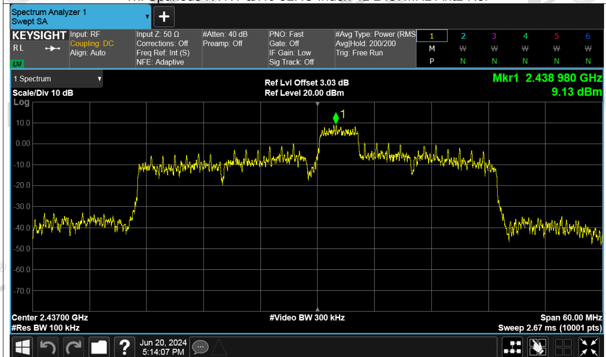
Tx. Spurious NVNT ax40 52RU Index 41 2437MHz Ant2 Emission
