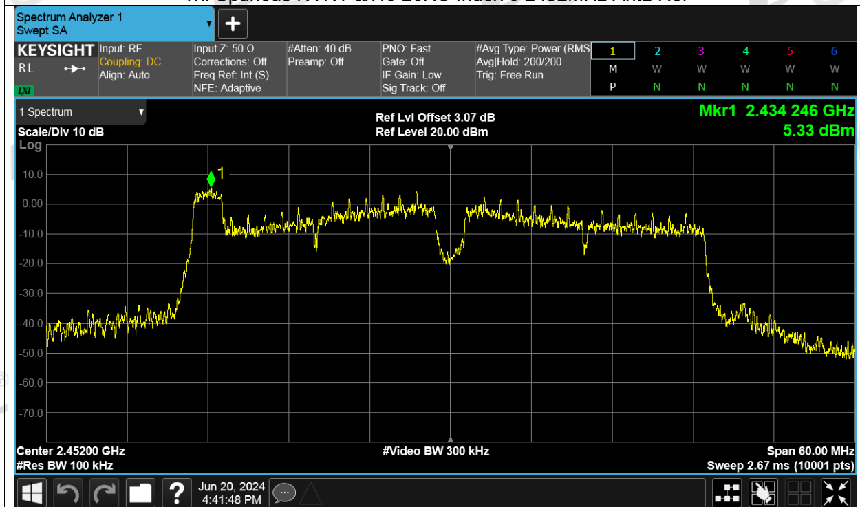
Tx. Spurious NVNT ax40 26RU Index 0 2452MHz Ant1 Emission
