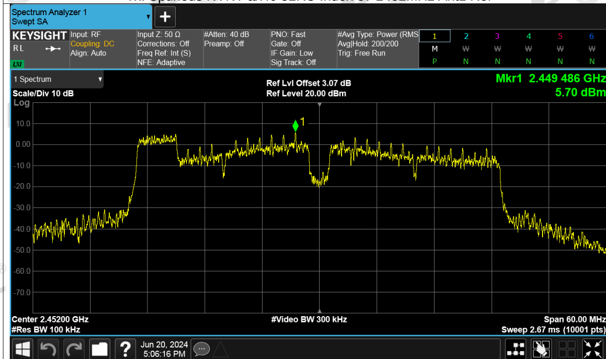
Tx. Spurious NVNT ax40 52RU Index 37 2452MHz Ant1 Emission
