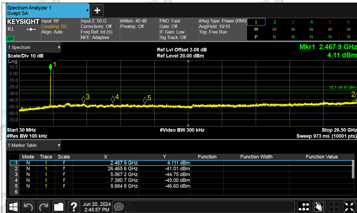
Tx. Spurious NVNT ax20 52RU Index 40 2462MHz Ant2 Ref
