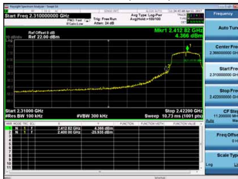
Mode 2 CH01(2412MHz)
