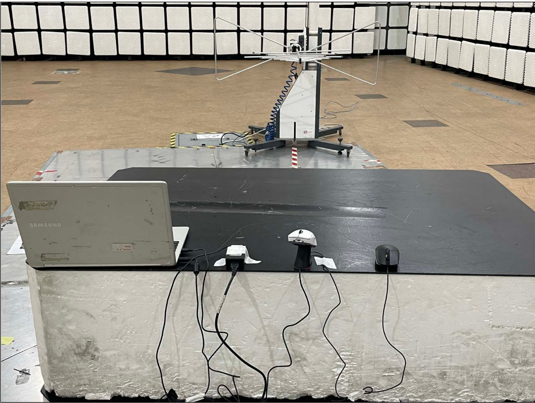
Radiated Emission _ Rear
