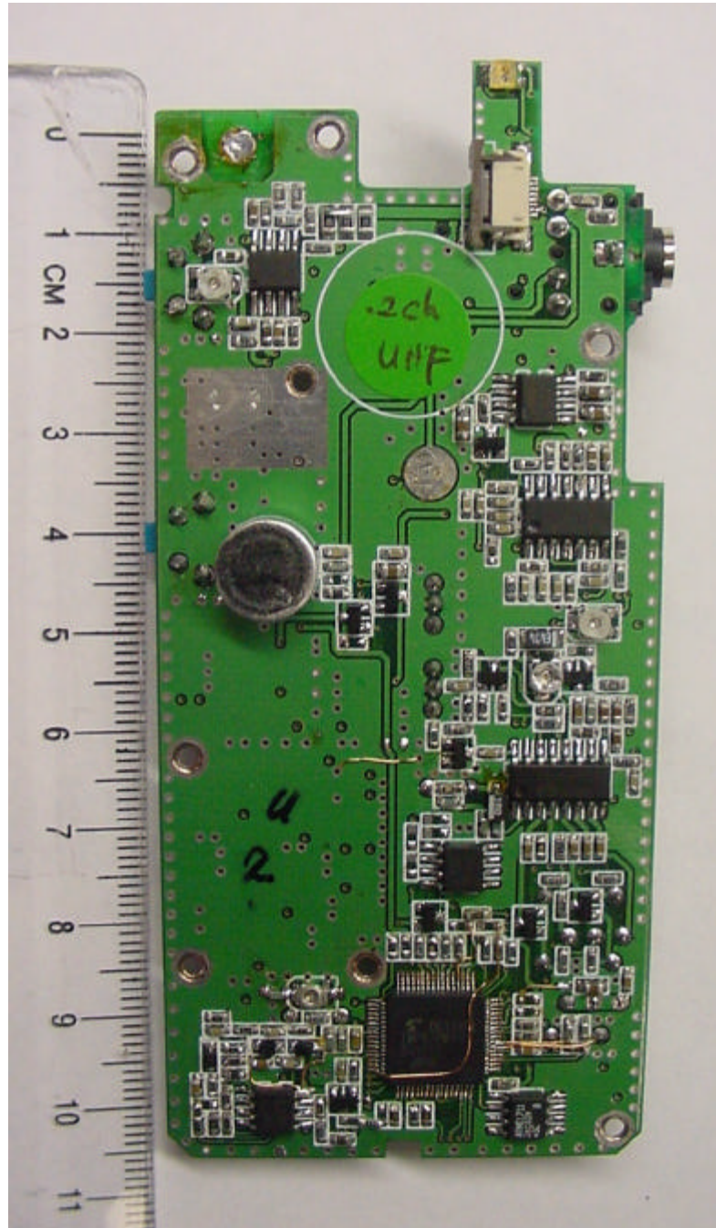
PHOTOGRAPH 5: FRONT VIEW OF PCB
