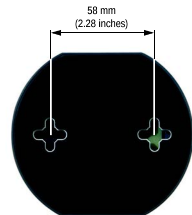
Figure 5-23: Wall-Mount Slots
