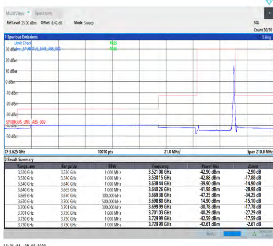
1-N48-PC3-30-30-H-5-CP-QPSK-Edge_1RB_Right-1 @77-Ant7-1--PASS-see graph
