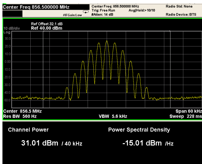
Mod. FM
