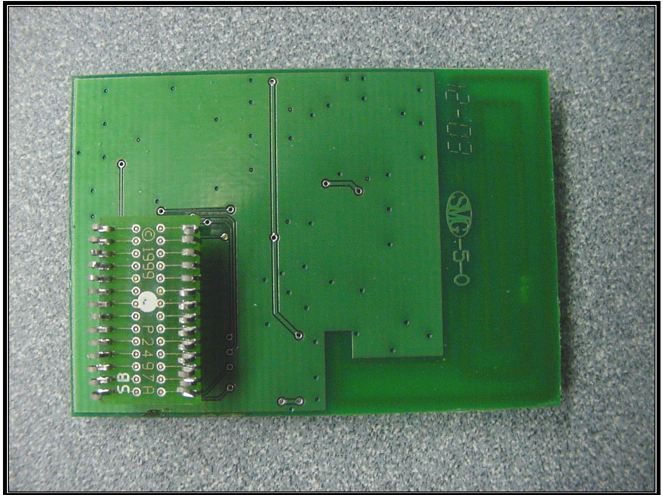
PHOTOGRAPH 14: CONNECTION SIDE OF SMALL PCB
