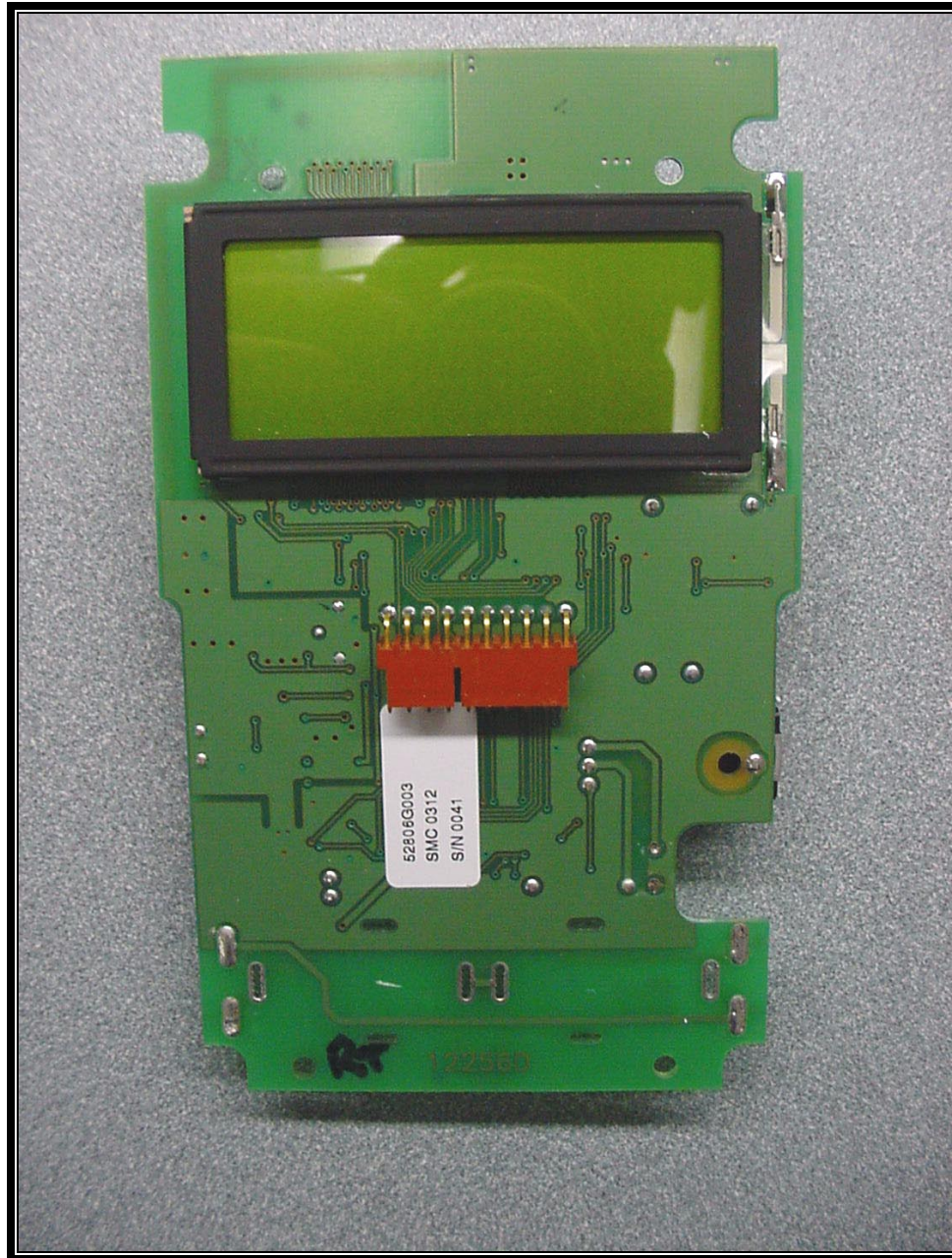
PHOTOGRAPH 11: FRONT VIEW OF MAIN PCB
