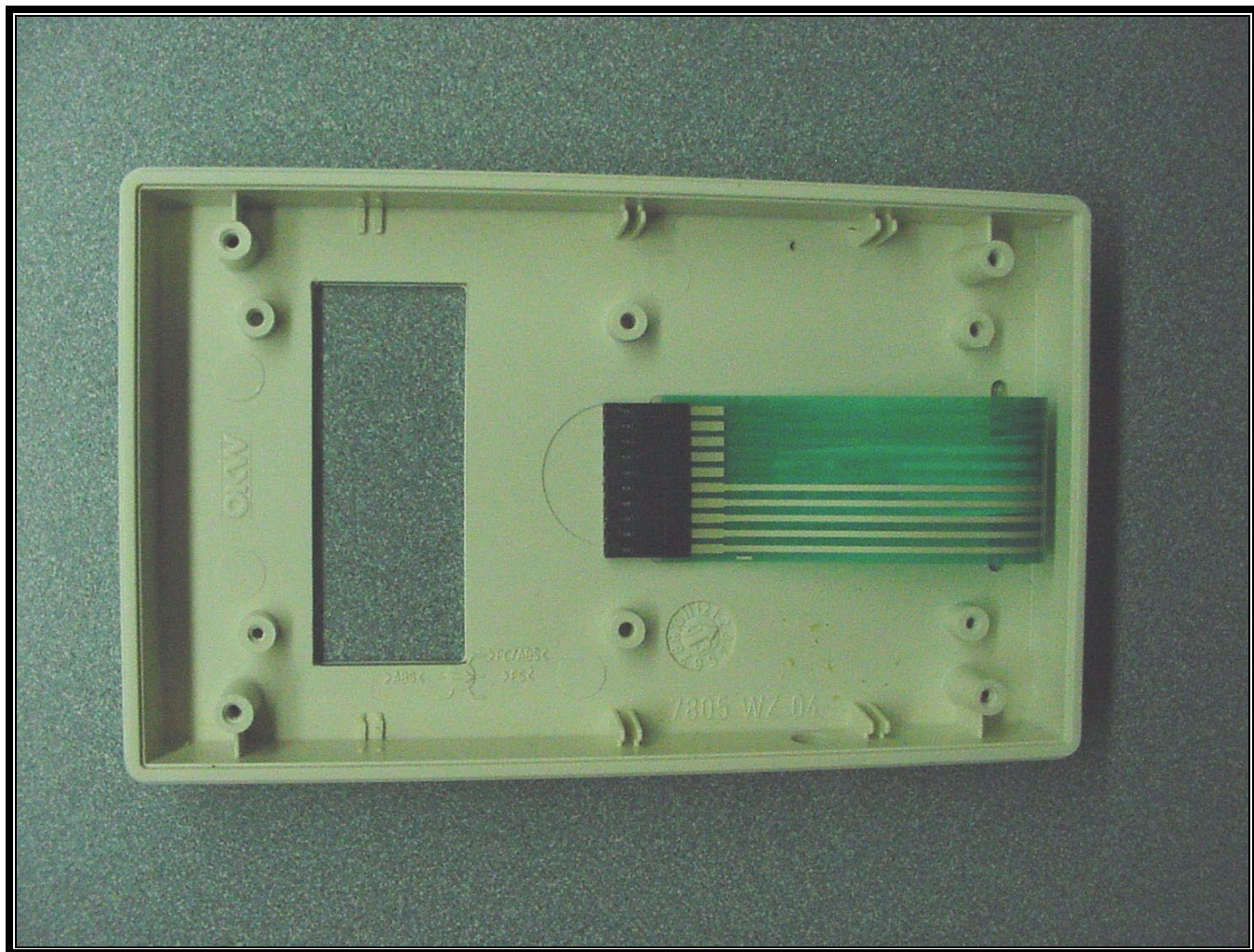
PHOTOGRAPH 15: INSIDE FRONT COVER
