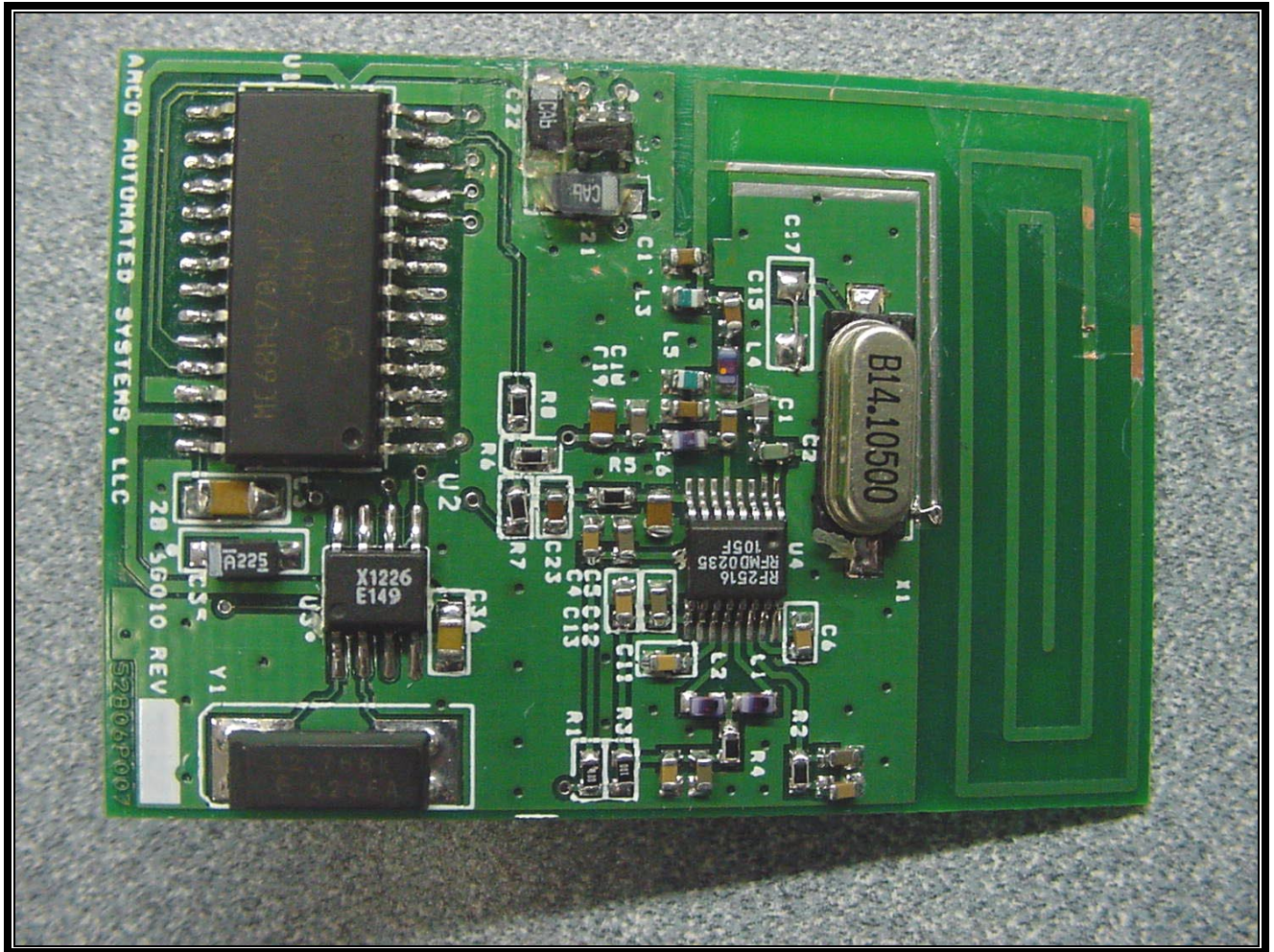
PHOTOGRAPH 13: COMPONENT SIDE OF SMALL PCB
