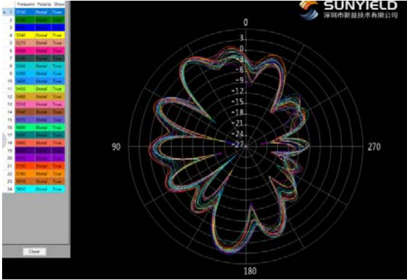
5G WIFI Phi=90deg
