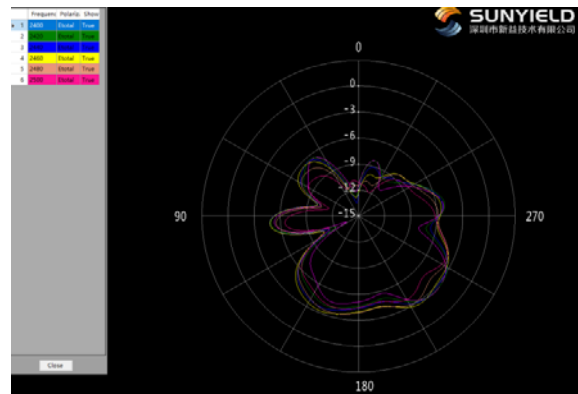
BT/2.4G WIFI \Phi=0^\circ
