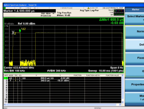
(Time per burst: 0.600ms*18pcs)
