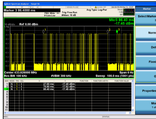
(Transmit cycle 59.4ms)
