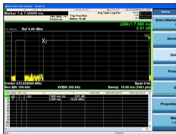
(Time per burst: 7.560ms*1pcs)
