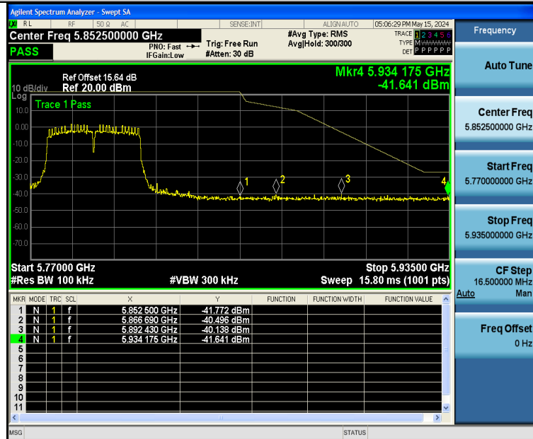
11AX40SISO-Ant1-5795-PASS
