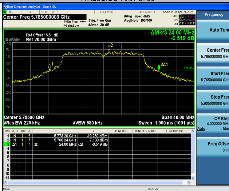
11N20SISO-Ant2-5785
