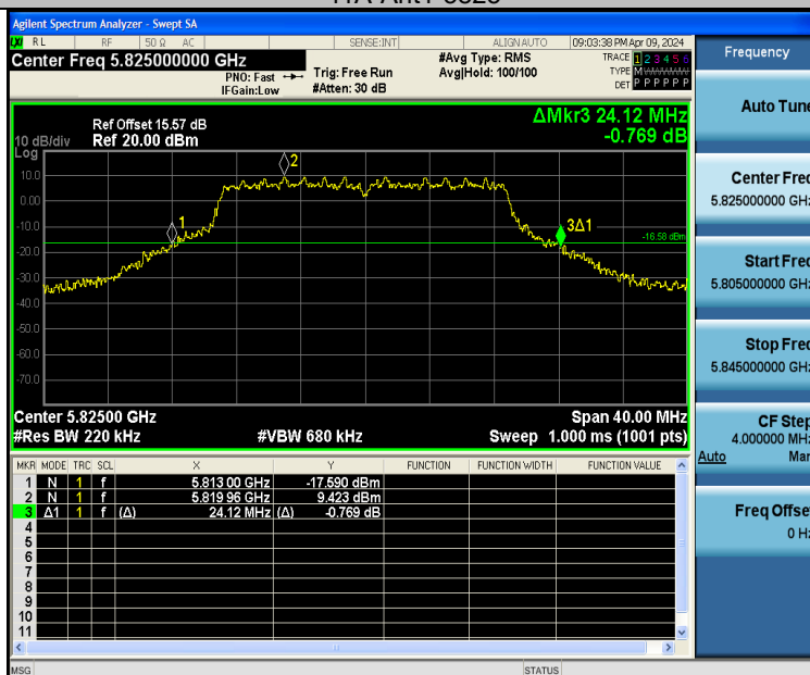
11A-Ant2-5825
