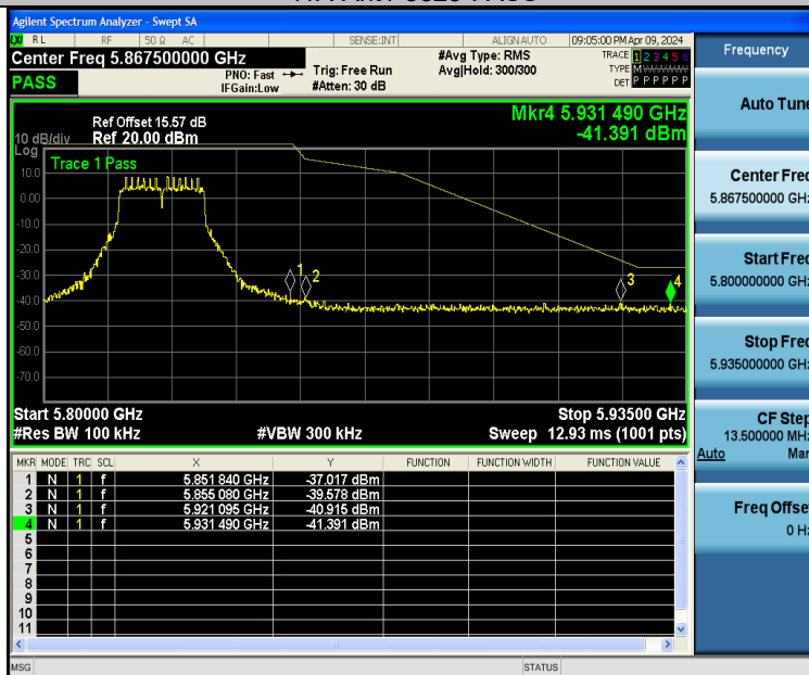
11A-Ant2-5825-PASS
