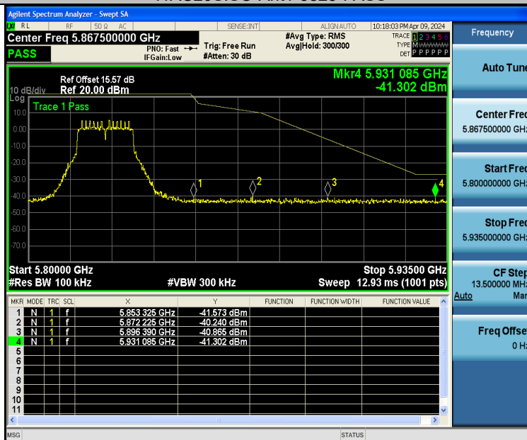
11AC20SISO-Ant2-5825-PASS
