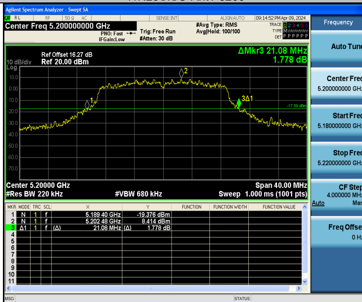
11N20SISO-Ant2-5200
