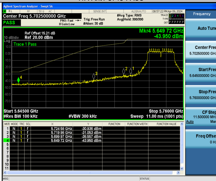
11A-Ant2-5745-PASS
