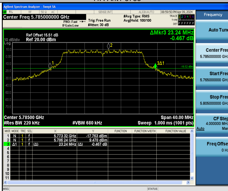
11A-Ant2-5785
