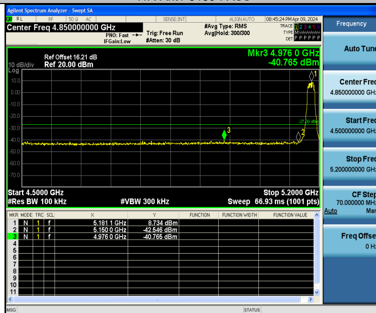
11A-Ant2-5180-PASS
