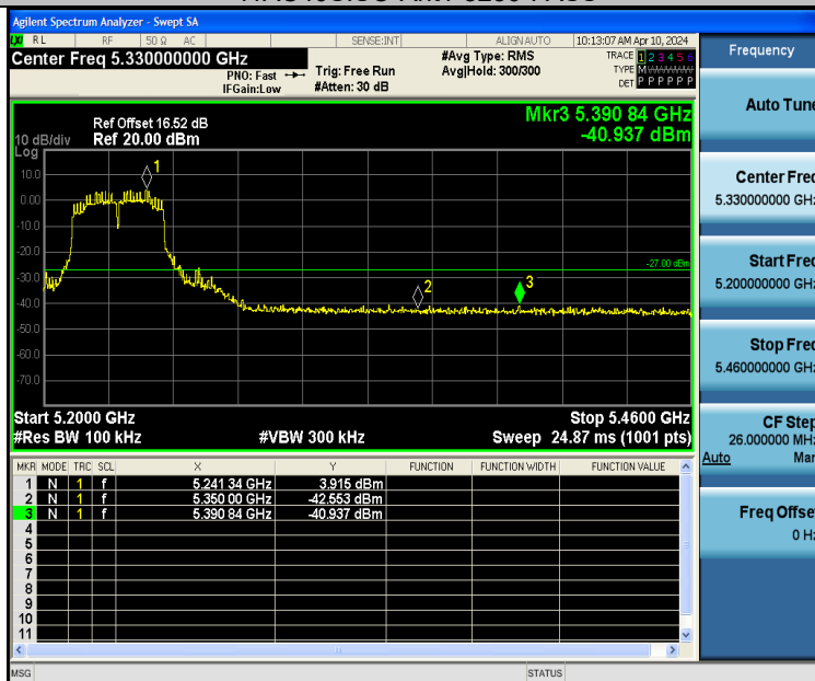
11AC40SISO-Ant2-5230-PASS
