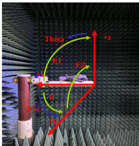
Figure 4: Geometry for SM-L310 for Radiation patterns.
