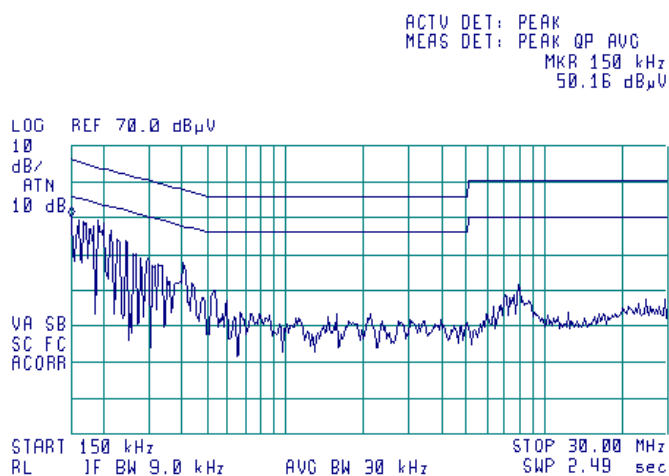
Plot 7.3.2 Conducted emission measurements
