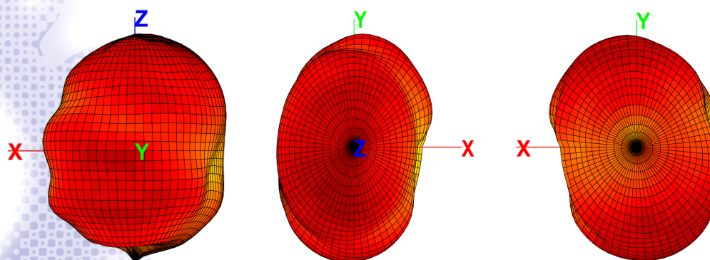
c) 2485 MHz (unit: dBi)
