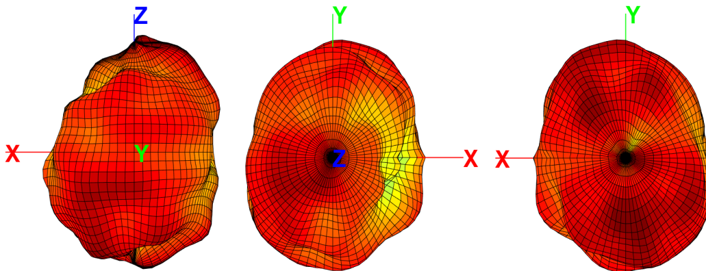
e) 5550 MHz (unit: dBi)
