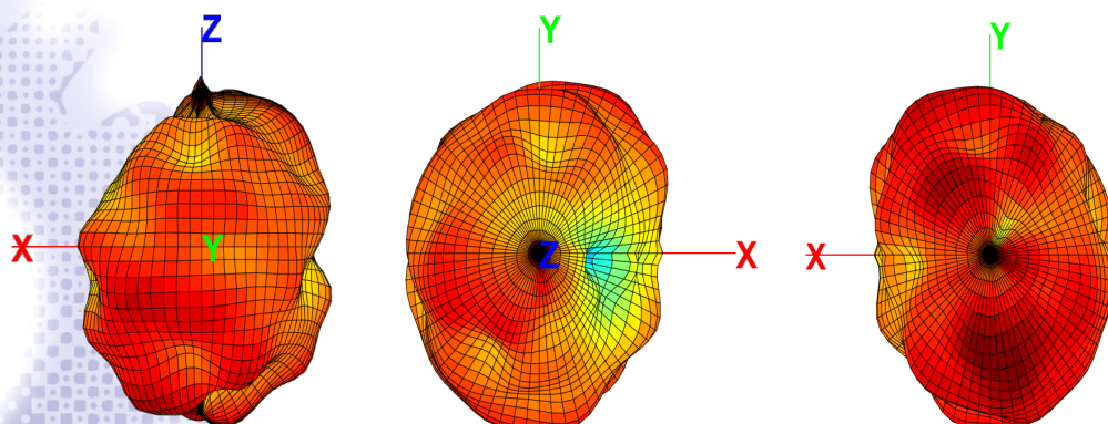
f) 5850 MHz (unit: dBi)
