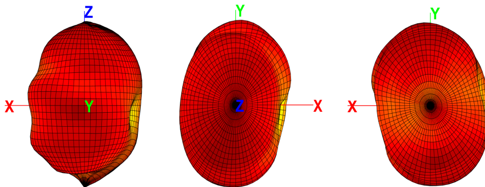
a) 2400 MHz (unit: dBi)
