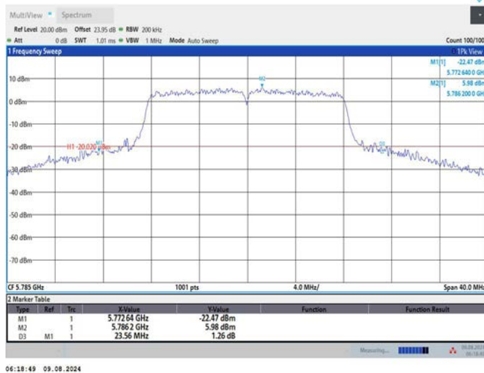
11A_Ant3_5785
