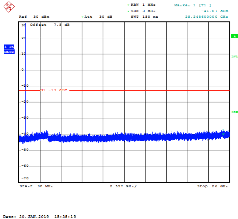
Fig.157 LTE band 26(Part 22): 30MHz – 26GHz
