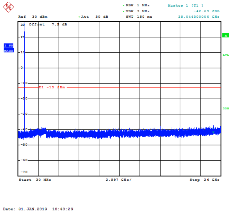
Fig.158 LTE band 26(Part 90): 30MHz – 26GHz
