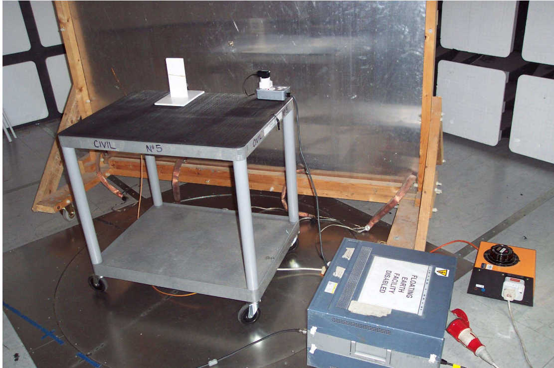
Sagem DC2006a – Test Set Up Photo 2 (Conducted Emissions)
