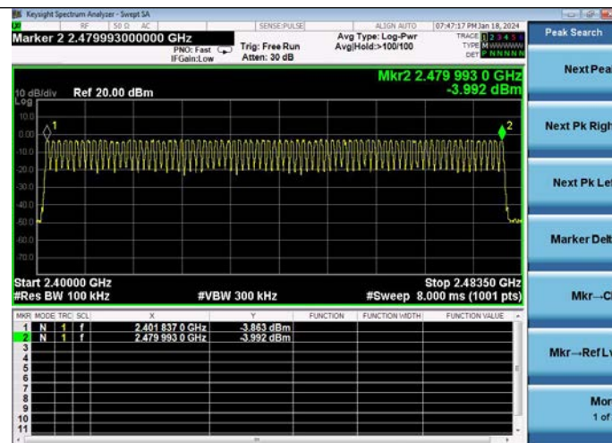
GFSK Modulation
