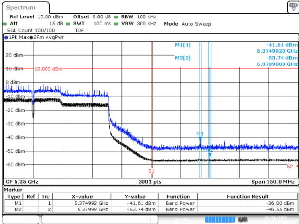
BE-R-HIGH, MIMO-A, 802.11ac160-VHT0, Ch50
