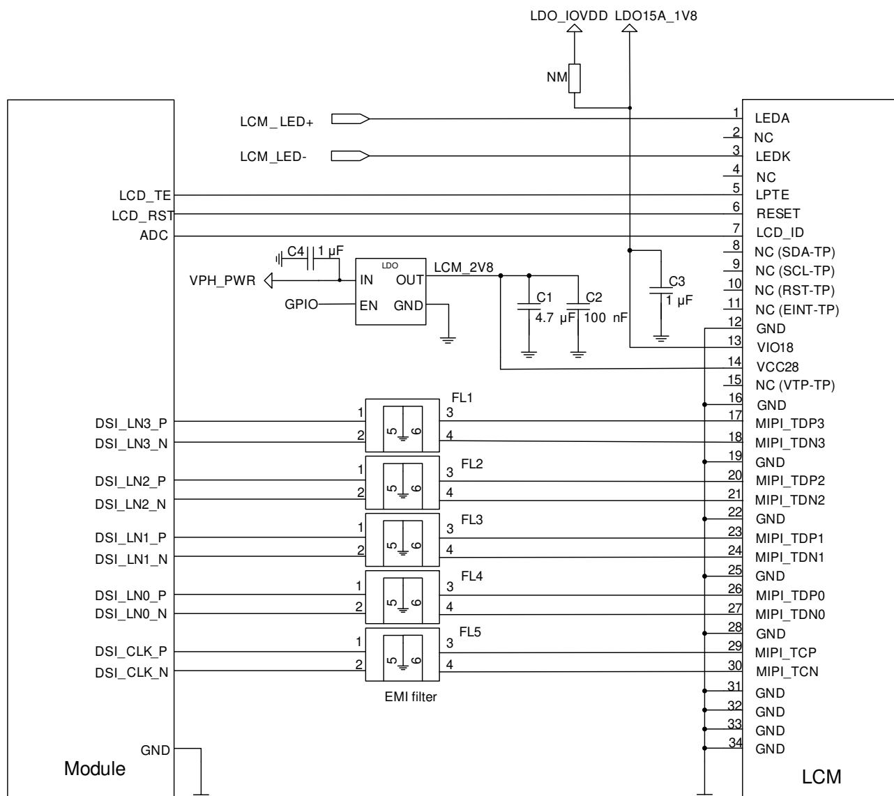
Figure 18: Reference Circuit Design for LCM Interface
