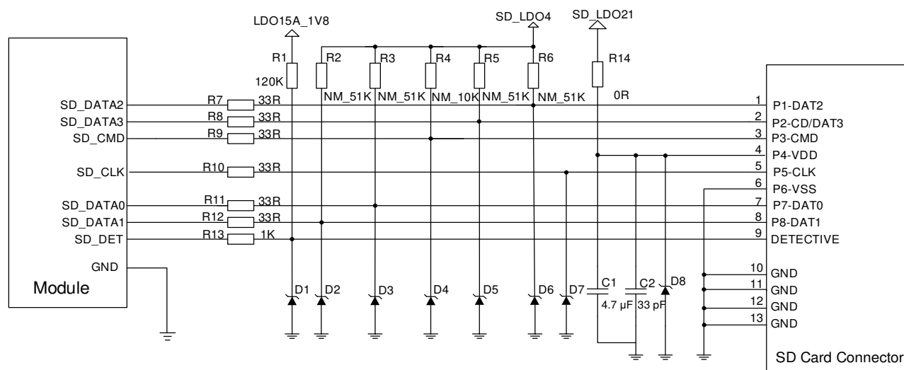
Figure 16: Reference Circuit for the SD Card Interface
