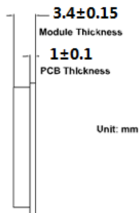
Figure 9-1 MHCBO5P-B Mechanical Dimension
