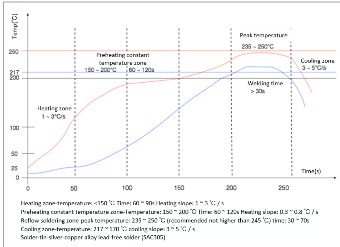
Figure 5-1 MHC805P-B Reflow temperature curve
