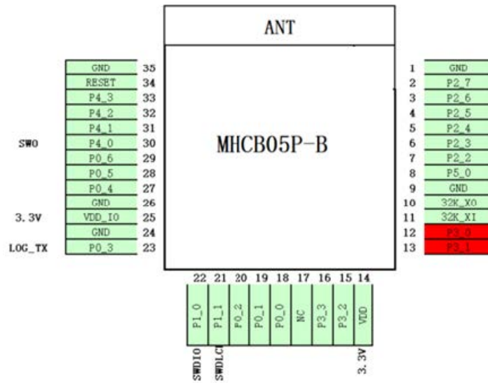
3-2 MHC805P-B pin definition description
