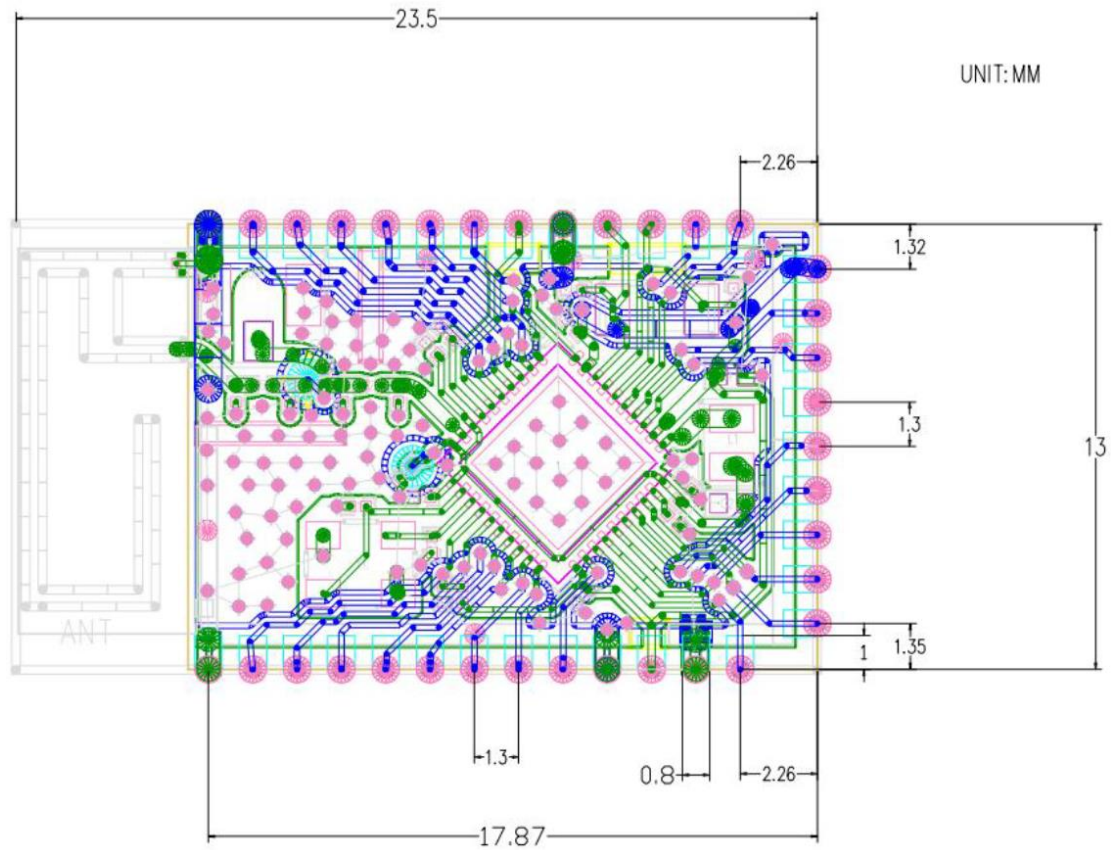
Figure 9-1 MHCBO5P-B Mechanical Dimension
