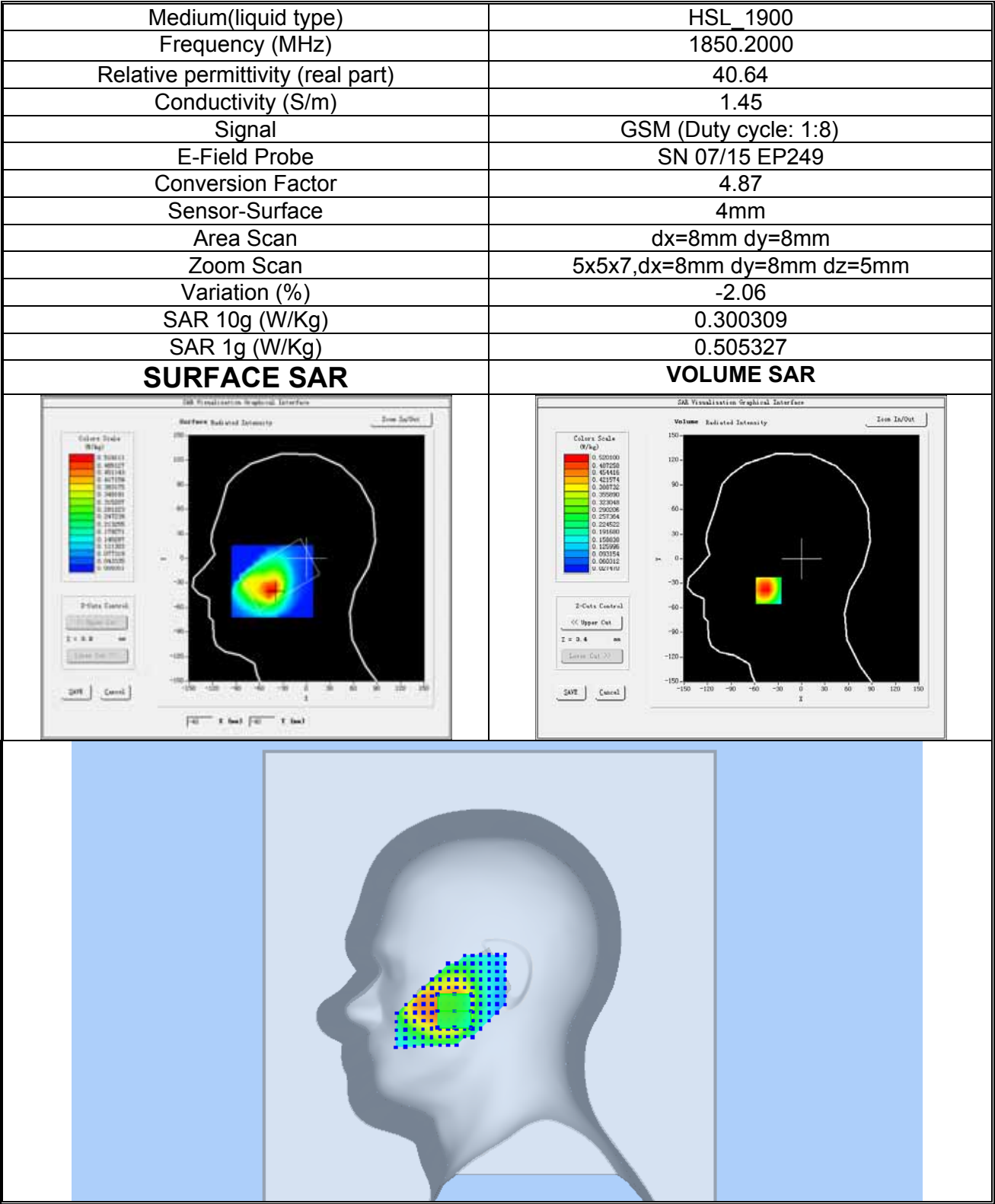
Plot 9: GSM1900, Low channel(Right Head, Cheek) Product Description: Feature Phone Urban Test Date: 2017-12-25
