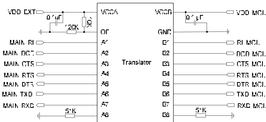
Figure 17: Main UART Reference Design (Translator Chip)
