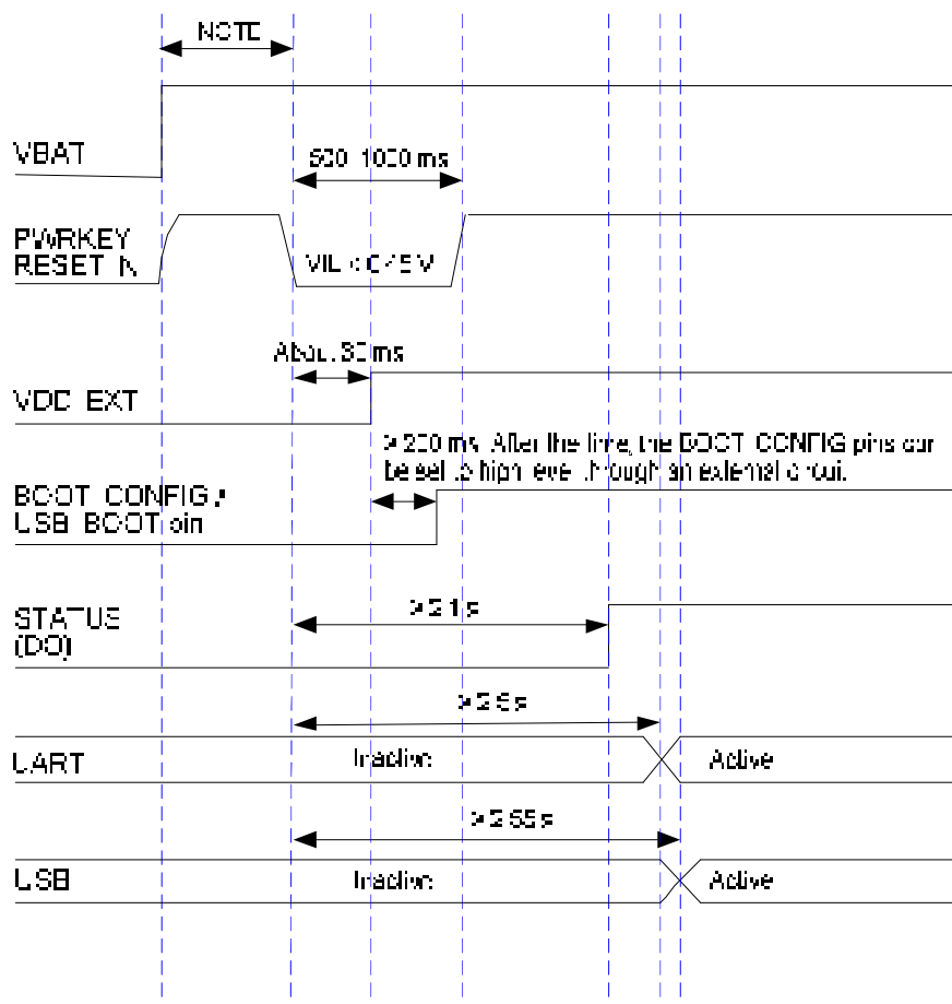
Figure 8: Power-on Timing
