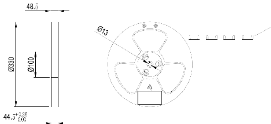
Figure 41: Reel Dimensions
