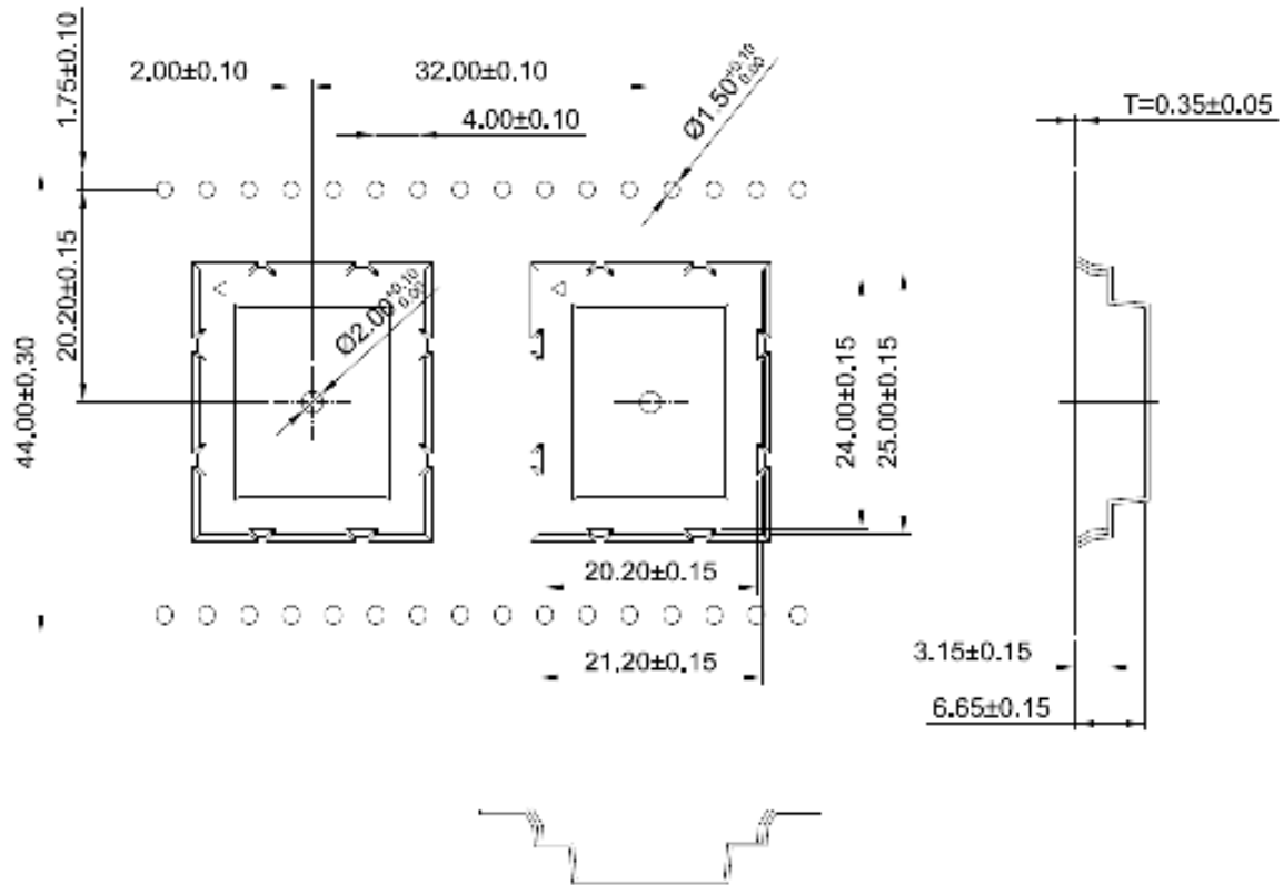
Figure 40: Tape Dimensions
