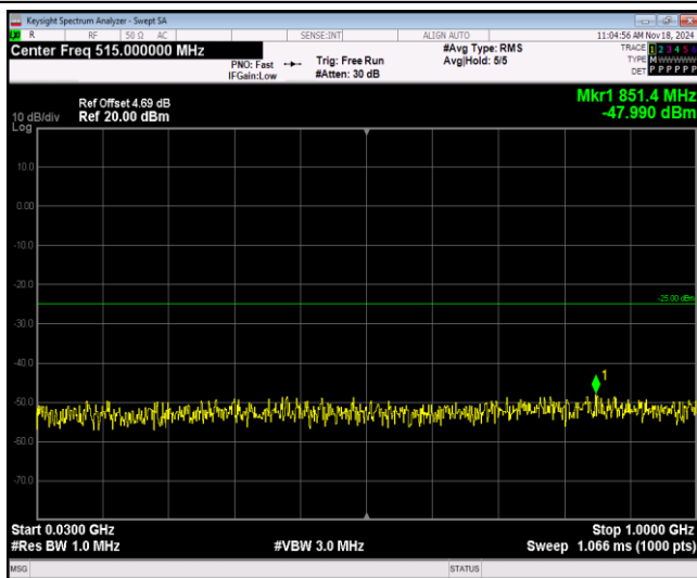
Band38-5MHz-16QAM-38000-1RB#0-Range1:30~10 00MHz
