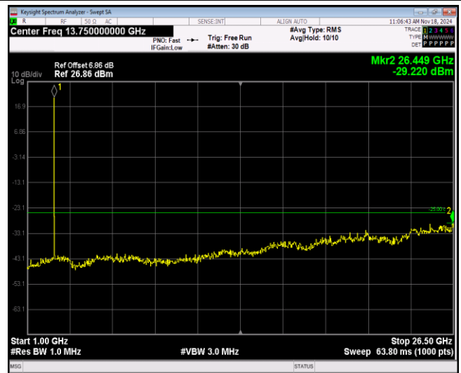
Band38-5MHz-16QAM-37775-1RB#0-Range2:1000~ 26500MHz
