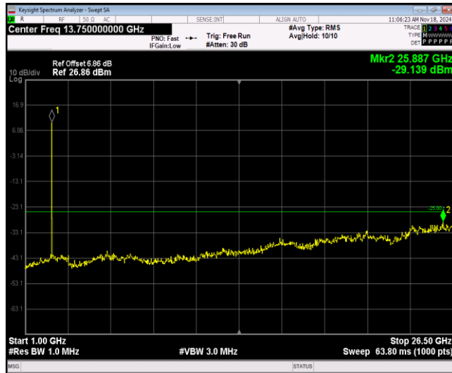
Band38-5MHz-64QAM-38225-1RB#0-Range2:1000~26500MHz
