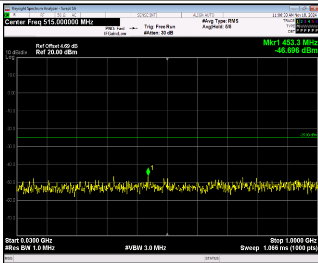
Band38-5MHz-16QAM-37775-1RB#0-Range1:30~10 00MHz
