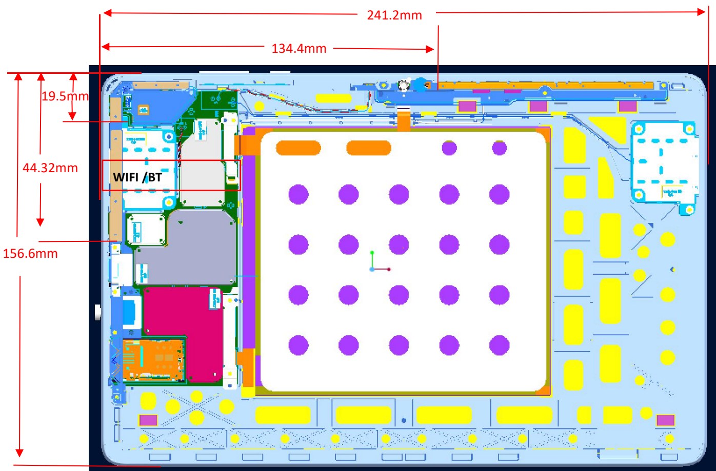
Antenna area diagram
