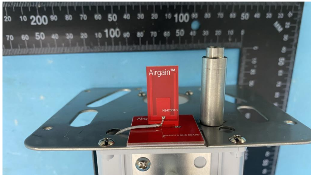
(5) EUT Photo (Wi-Fi Antenna)
