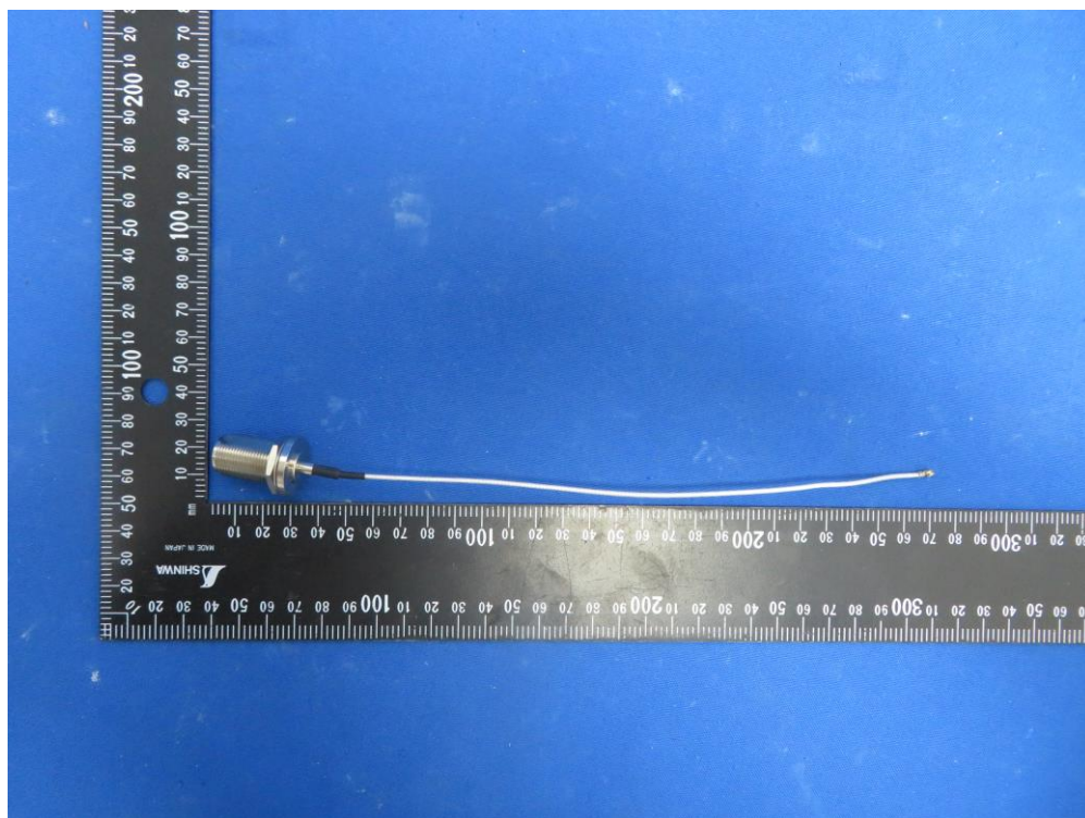
(6) EUT Photo (IPEX to N-type)
