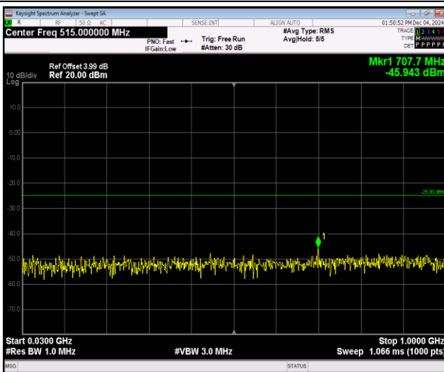
Band7-5MHz-64QAM-21425-1RB#0-Range1:30~100 0MHz
