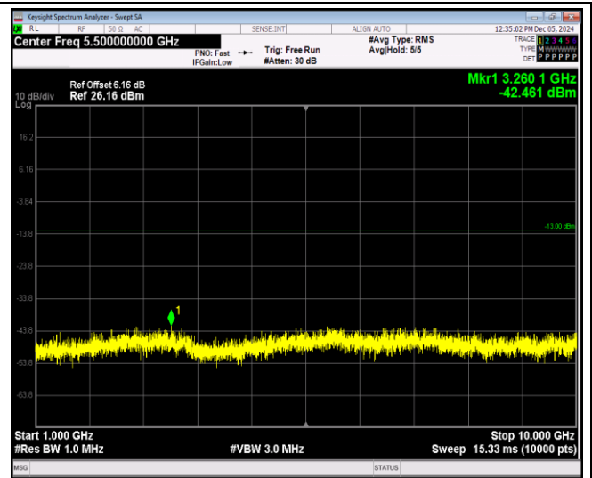
Band12-10MHz-QPSK-23130-1RB#0-Range2:1000~10000MHz
