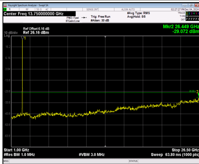
Band7-20MHz-64QAM-21350-1RB#0-Range2:1000~26500MHz
