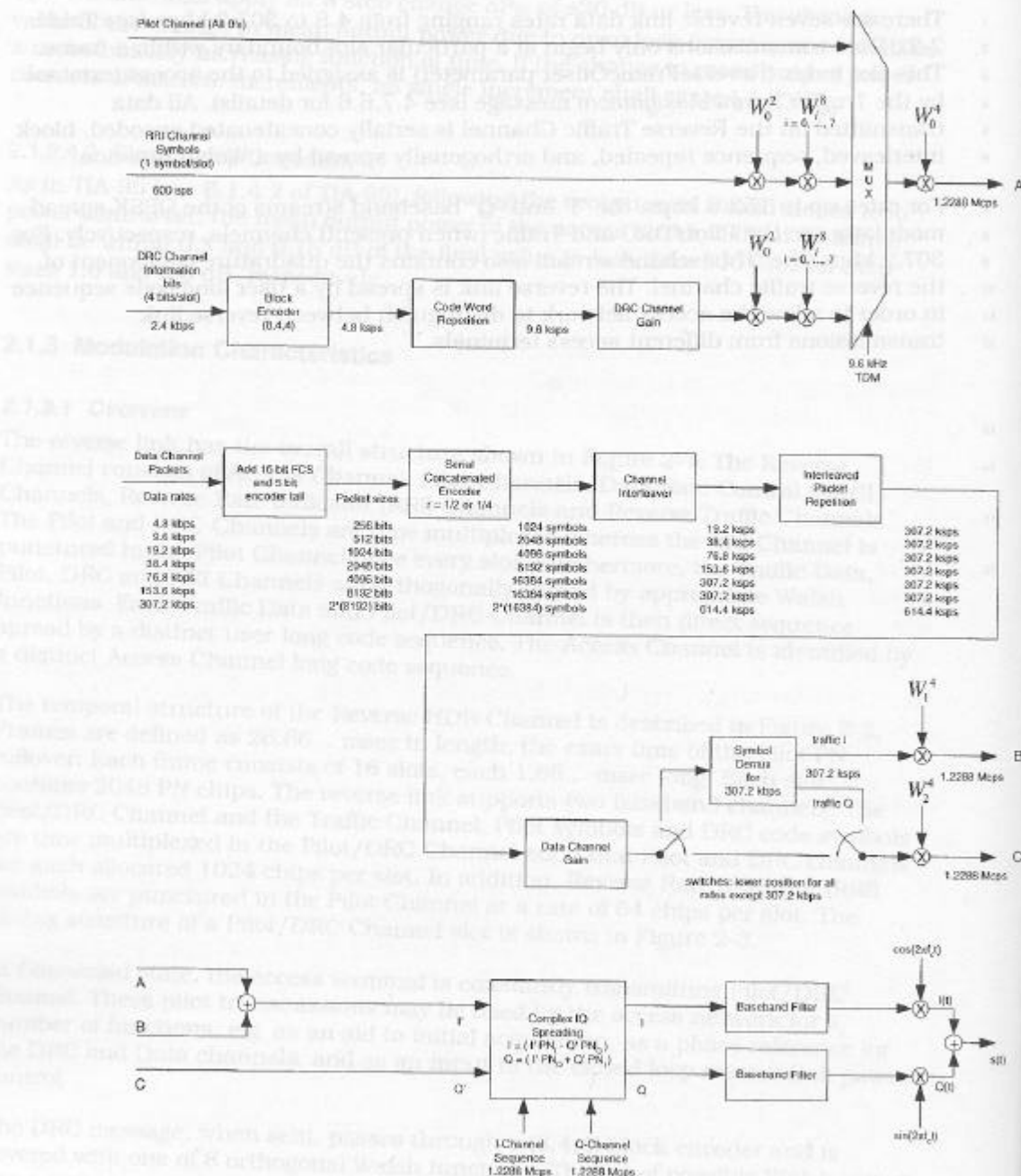
Figure 2-1 Reverse HDR Channel Structure 4
