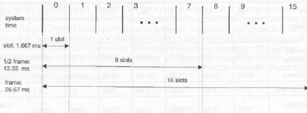
Figure 2-2 Reverse Link Frame Alignment
