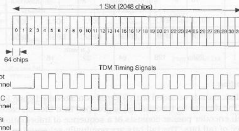
Figure 2-3 Slot Timing of Pilot/DRC Channel
