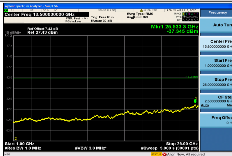
Band12-10MHz-16QAM-23095-1RB#0-1000~26000MHz
