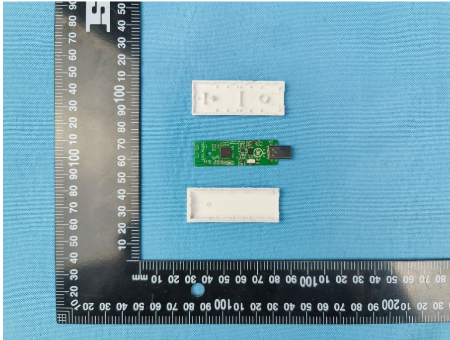
Photo 1: PCB view
