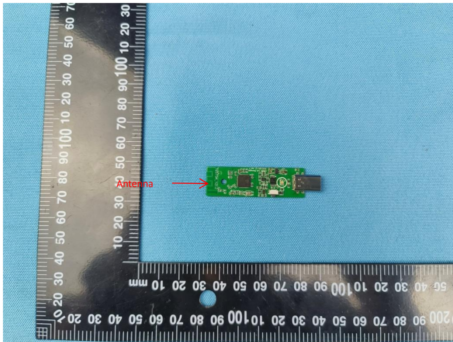
Photo 2: PCB view
