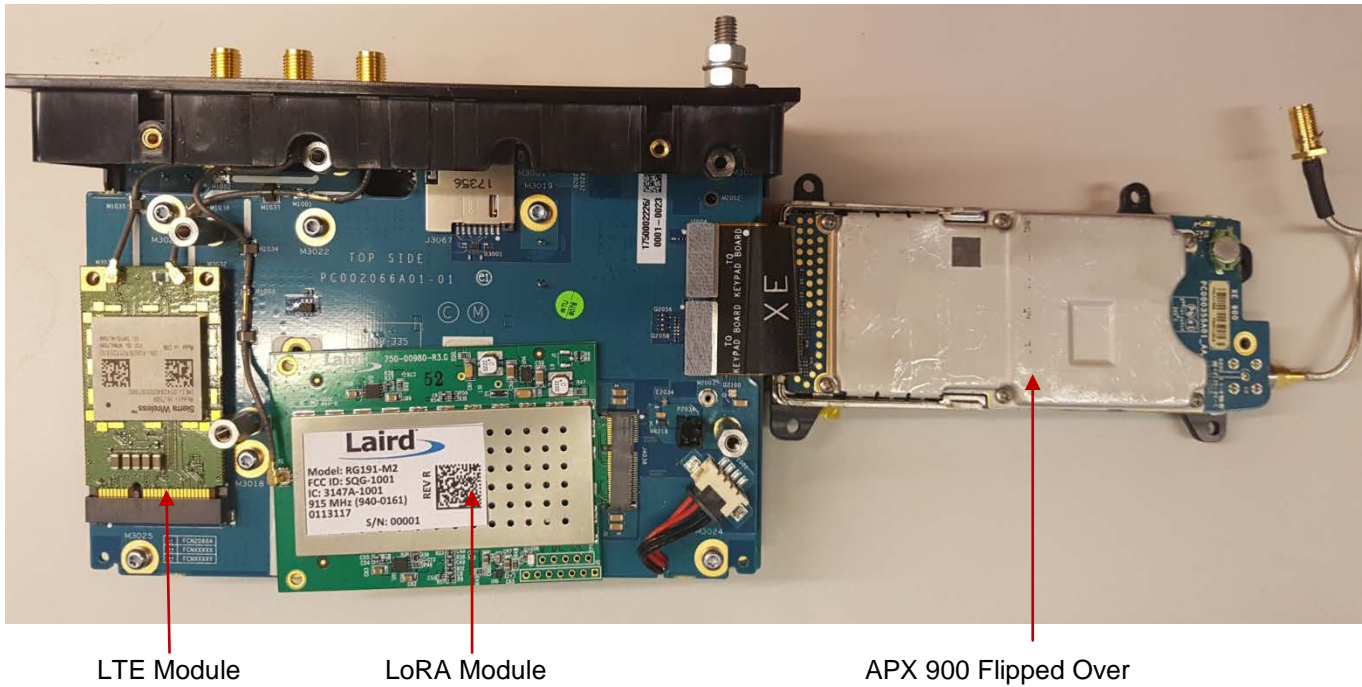
MC-EDGE Piggy Board Top View With Front Panel (APX4000 900 Flipped over, with LORA and LTE)
