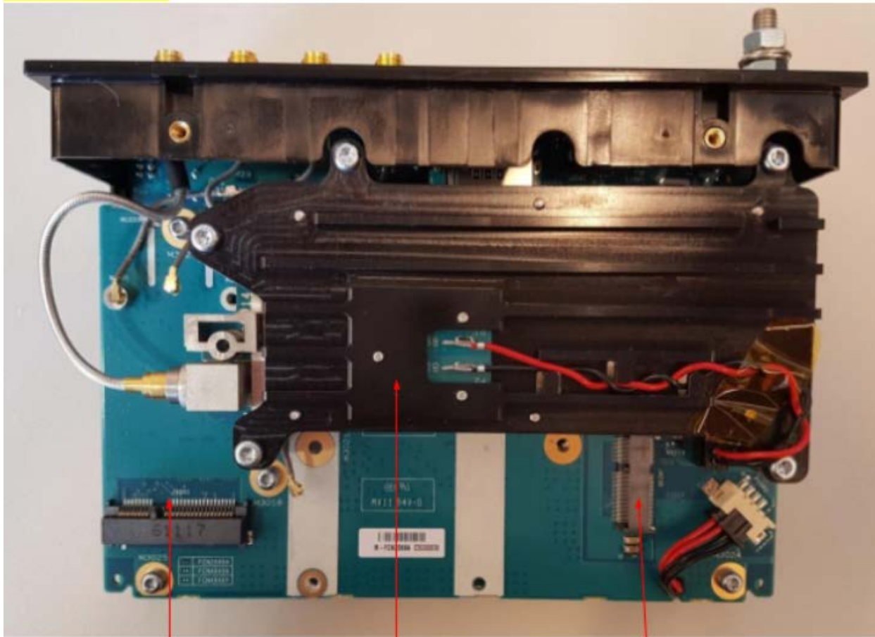
MC-EDGE Piggy Board Top View With Front Panel (APX4000 900 Installed)
