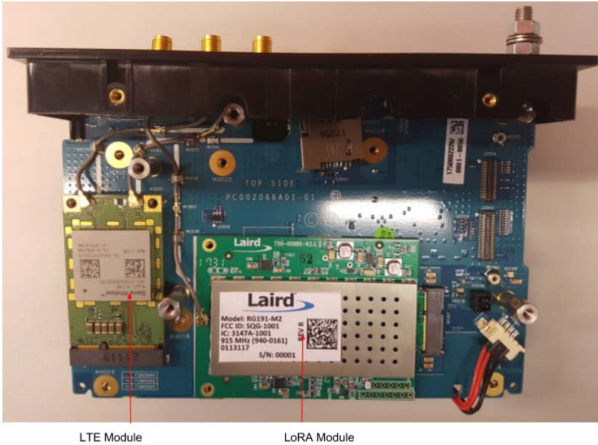
MC-EDGE Piggy Board Top View With Front Panel (APX4000 900 Removed, with LORA and LTE)
