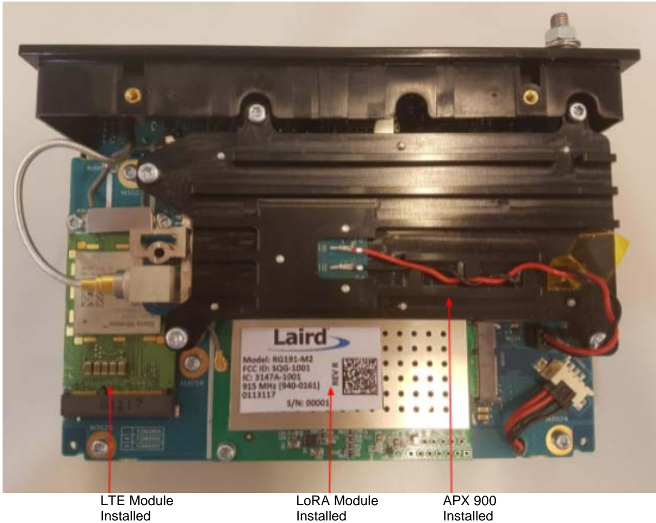
MC-EDGE Piggy Board Top View With Front Panel (APX4000 900 Installed, with LORA and LTE)
